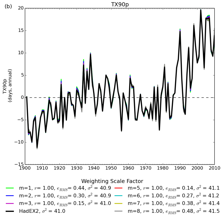
Figure 2: The time series for global average TX90p showing the different curves for the different weighting values (colours are indicated below the plot). The figure also shows the correlation coefficient ( r ), variance ( \sigma^2 ) and root-mean-square error ( e_{RMS} ) between each series and HadEX2. All choices have been normalised over the 1961-1990 period.
