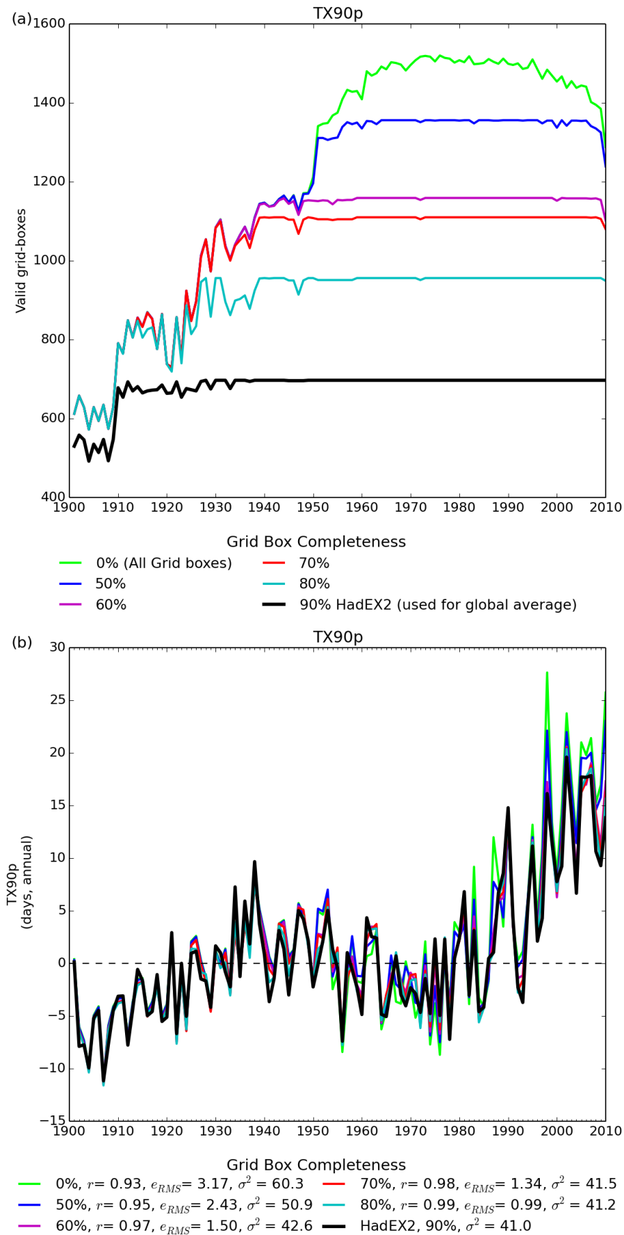
Figure 1: (a) The coverage, showing the different curves for different completeness requirements, for TX90p. The total coverage is shown the curve in light green, whereas the coverage used when calculating global averages is in black, with a range of other completeness percentages shown in between. (b) : The time series for global average of TX90p. Also shown are the comparison of other completenesses to that used in HadEX2 (90 %) using the correlation coefficient, r , the root mean square error e_{ems} and the variance, \sigma^2 .
