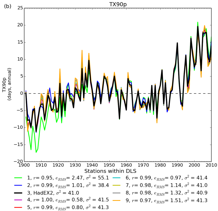
Figure 3: (a) : The number of non-missing grid boxes for TX90p showing the different curves for left numbers of stations within a DLS of the grid box centre. Note that the global average only takes grid boxes which have 90 per cent completeness or more, whereas all grid boxes are shown in the coverage series. (b) : The time series for global average TX90p.
