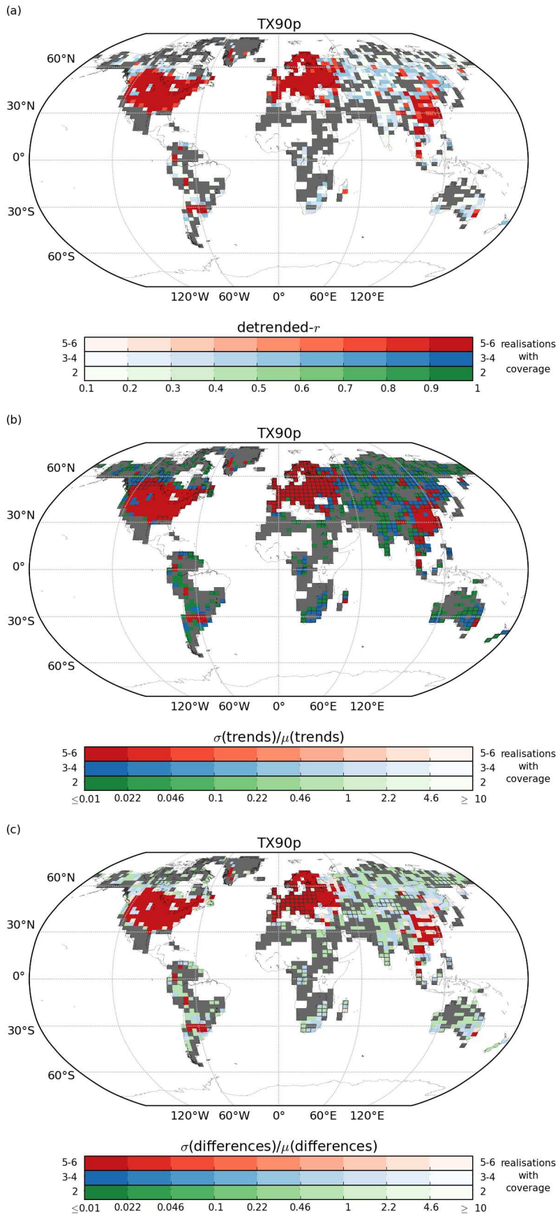
Figure 6: As for Fig. 4 but for TX90p restricted by the number of stations within a grid box. Grey grid boxes are those where only one of the 6 possible stations per grid box choices results in a value, green when 2, blue when 3-4 and red when 5-6 of the possible choices result in a value. Note that the HadEX2 method does not require any stations to be present within a grid box for a value to be calculated. In (b) and (c), boxes which have been outlined are ones where the trend was significant in the HadEX2 version. For details on the calculation method, see text.
