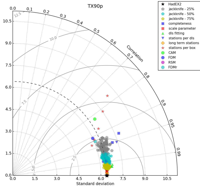
Figure 19: The Taylor Diagram for TX90p calculated using the global average timeseries for each choice. Each of the different methodological choices are shown using a different symbol and colour as indicated in the legend.
