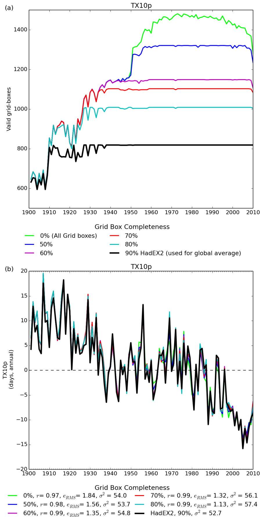
Figure 1: (a) The coverage, showing the different curves for different completeness requirements, for TX10p. The total coverage is shown the curve in light green, whereas the coverage used when calculating global averages is in black, with a range of other completeness percentages shown in between. (b) : The time series for global average of TX10p. Also shown are the comparison of other completenesses to that used in HadEX2 (90 %) using the correlation coefficient, r , the root mean square error e_{ems} and the variance, \sigma^2 .
