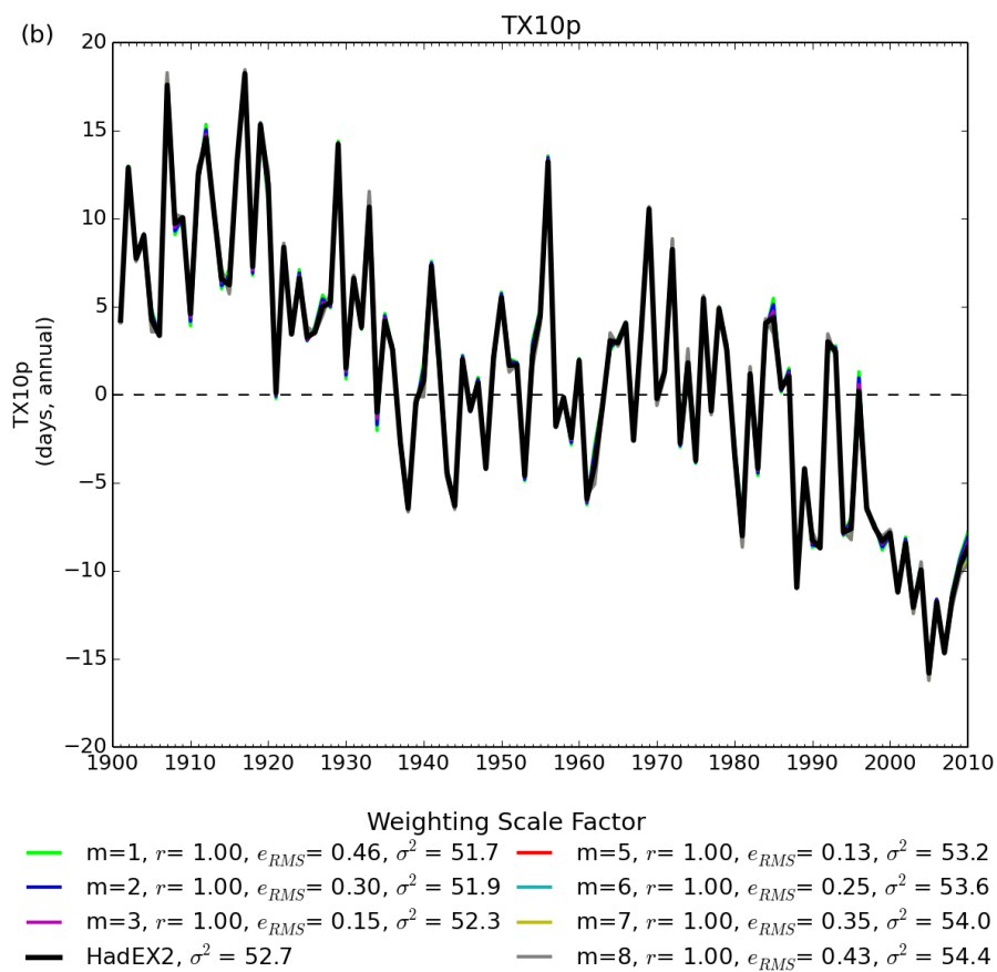
Figure 2: The time series for global average TX10p showing the different curves for the different weighting values (colours are indicated below the plot). The figure also shows the correlation coefficient ( r ), variance ( \sigma^2 ) and root-mean-square error ( e_{RMS} ) between each series and HadEX2. All choices have been normalised over the 1961-1990 period.
