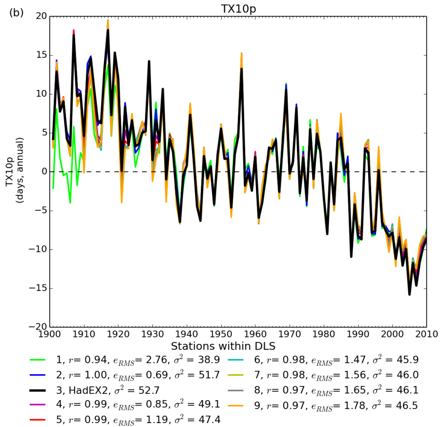
Figure 3: (a) : The number of non-missing grid boxes for TX10p showing the different curves for left numbers of stations within a DLS of the grid box centre. Note that the global average only takes grid boxes which have 90 per cent completeness or more, whereas all grid boxes are shown in the coverage series. (b) : The time series for global average TX10p.
