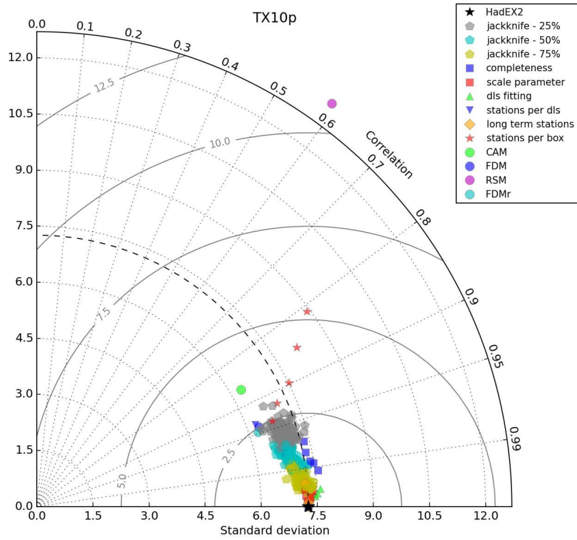
Figure 19: The Taylor Diagram for TX10p calculated using the global average timeseries for each choice. Each of the different methodological choices are shown using a different symbol and colour as indicated in the legend.
