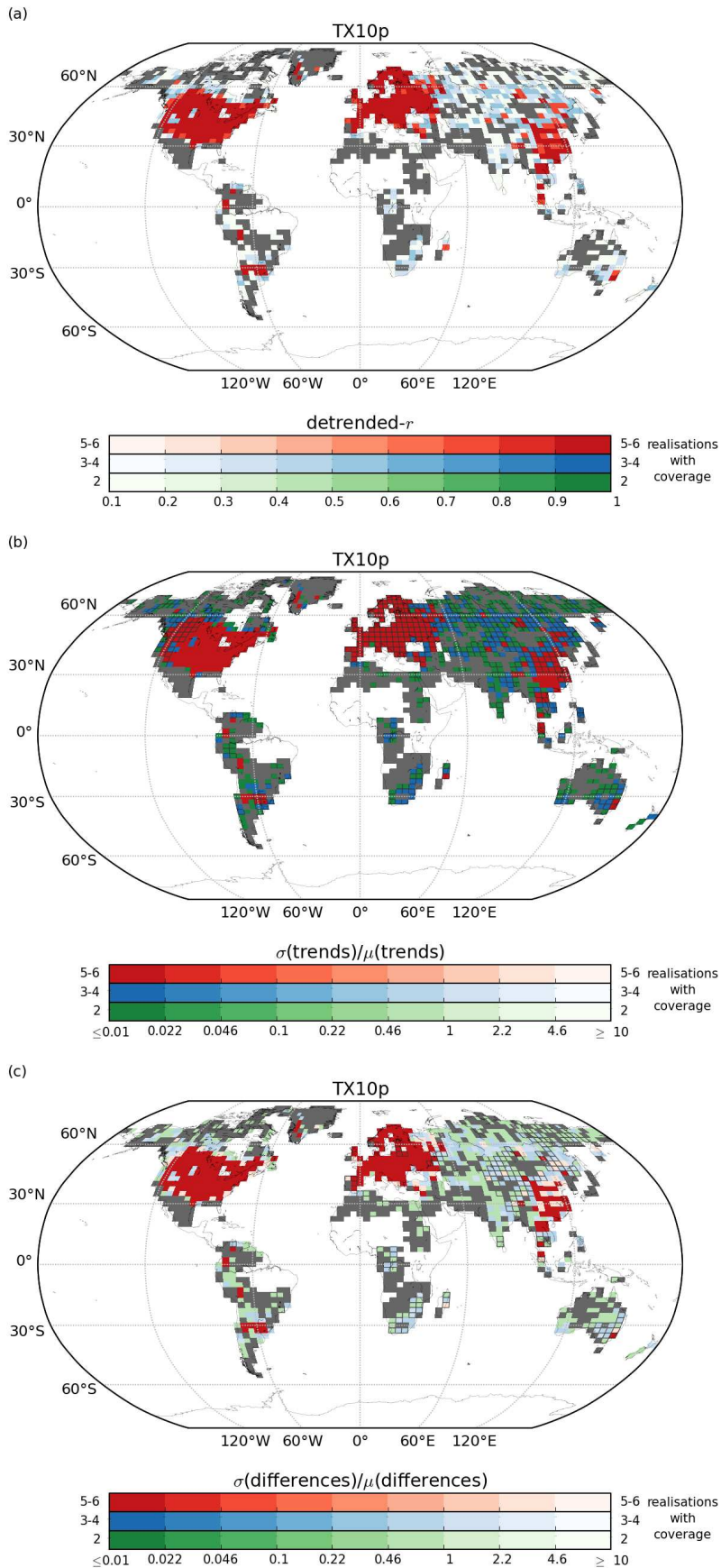
Figure 6: As for Fig. 4 but for TX10p restricted by the number of stations within a grid box. Grey grid boxes are those where only one of the 6 possible stations per grid box choices results in a value, green when 2, blue when 3-4 and red when 5-6 of the possible choices result in a value. Note that the HadEX2 method does not require any stations to be present within a grid box for a value to be calculated. In (b) and (c), boxes which have been outlined are ones where the trend was significant in the HadEX2 version. For details on the calculation method, see text.
