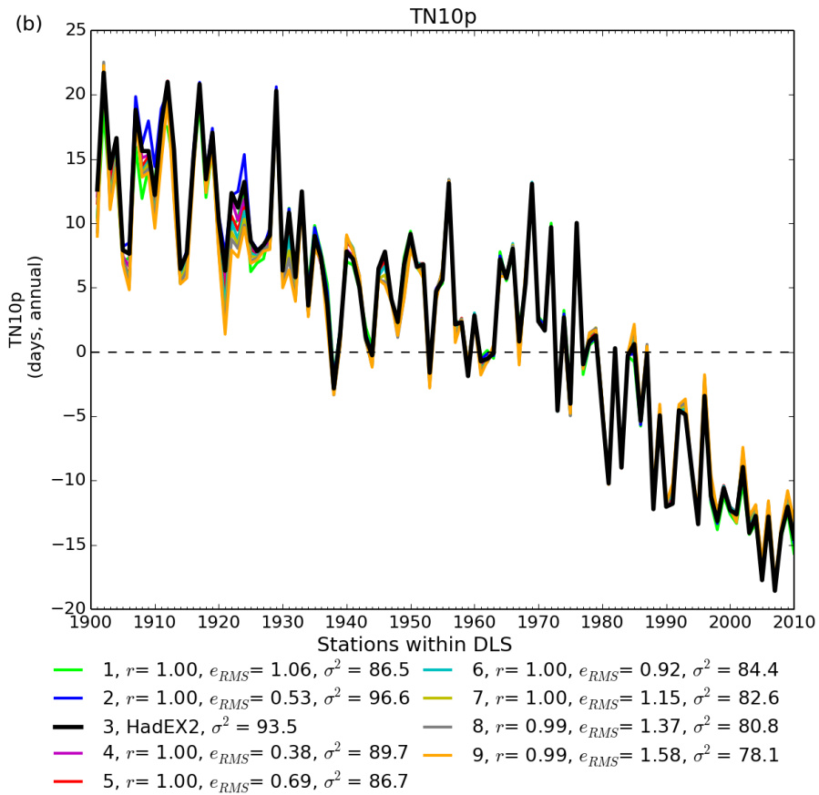
Figure 3: (a) : The number of non-missing grid boxes for TN10p showing the different curves for left numbers of stations within a DLS of the grid box centre. Note that the global average only takes grid boxes which have 90 per cent completeness or more, whereas all grid boxes are shown in the coverage series. (b) : The time series for global average TN10p.
