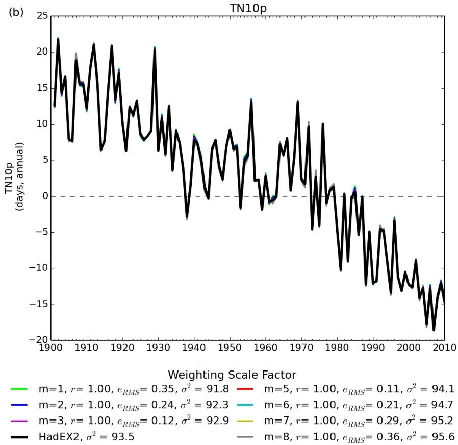
Figure 2: The time series for global average TN10p showing the different curves for the different weighting values (colours are indicated below the plot). The figure also shows the correlation coefficient ( r ), variance ( \sigma^2 ) and root-mean-square error ( e_{RMS} ) between each series and HadEX2. All choices have been normalised over the 1961-1990 period.
