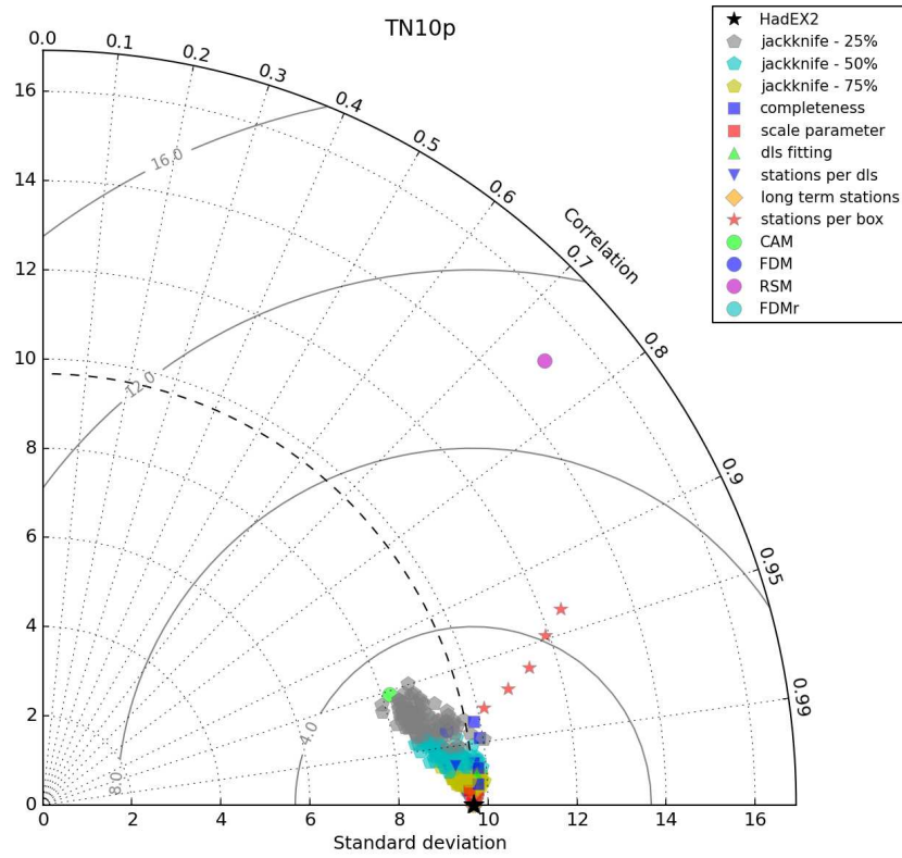
Figure 19: The Taylor Diagram for TN10p calculated using the global average timeseries for each choice. Each of the different methodological choices are shown using a different symbol and colour as indicated in the legend.
