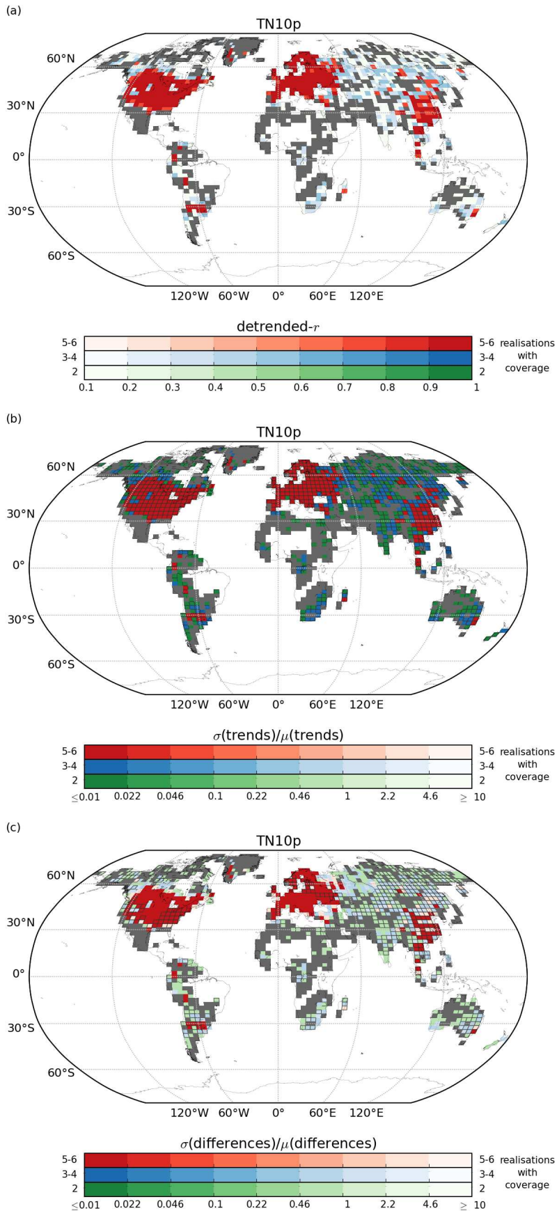
Figure 6: As for Fig. 4 but for TN10p restricted by the number of stations within a grid box. Grey grid boxes are those where only one of the 6 possible stations per grid box choices results in a value, green when 2, blue when 3-4 and red when 5-6 of the possible choices result in a value. Note that the HadEX2 method does not require any stations to be present within a grid box for a value to be calculated. In (b) and (c), boxes which have been outlined are ones where the trend was significant in the HadEX2 version. For details on the calculation method, see text.
