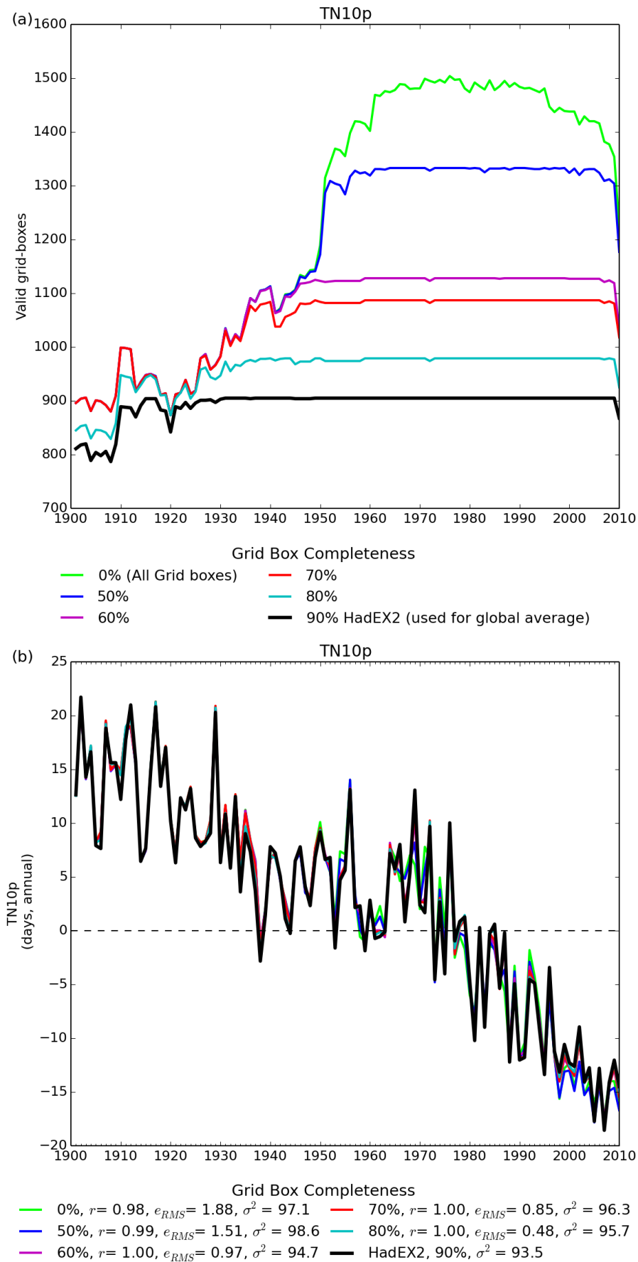
Figure 1: (a) The coverage, showing the different curves for different completeness requirements, for TN10p. The total coverage is shown the curve in light green, whereas the coverage used when calculating global averages is in black, with a range of other completeness percentages shown in between. (b) : The time series for global average of TN10p. Also shown are the comparison of other completenesses to that used in HadEX2 (90 %) using the correlation coefficient, r , the root mean square error e_{ems} and the variance, \sigma^2 .
