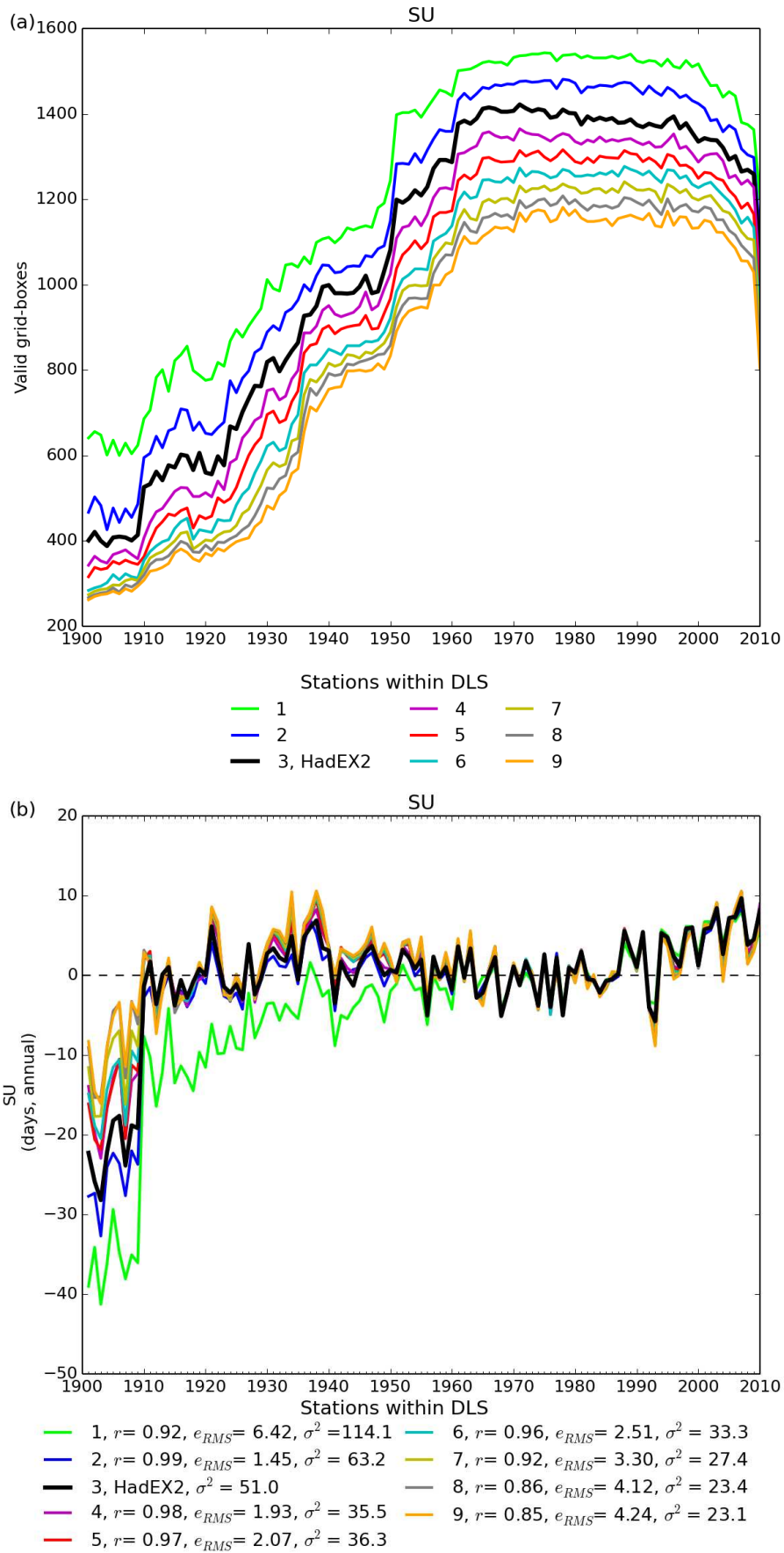
Figure 3: (a) : The number of non-missing grid boxes for SU showing the different curves for left numbers of stations within a DLS of the grid box centre. Note that the global average only takes grid boxes which have 90 per cent completeness or more, whereas all grid boxes are shown in the coverage series. (b) : The time series for global average SU.
