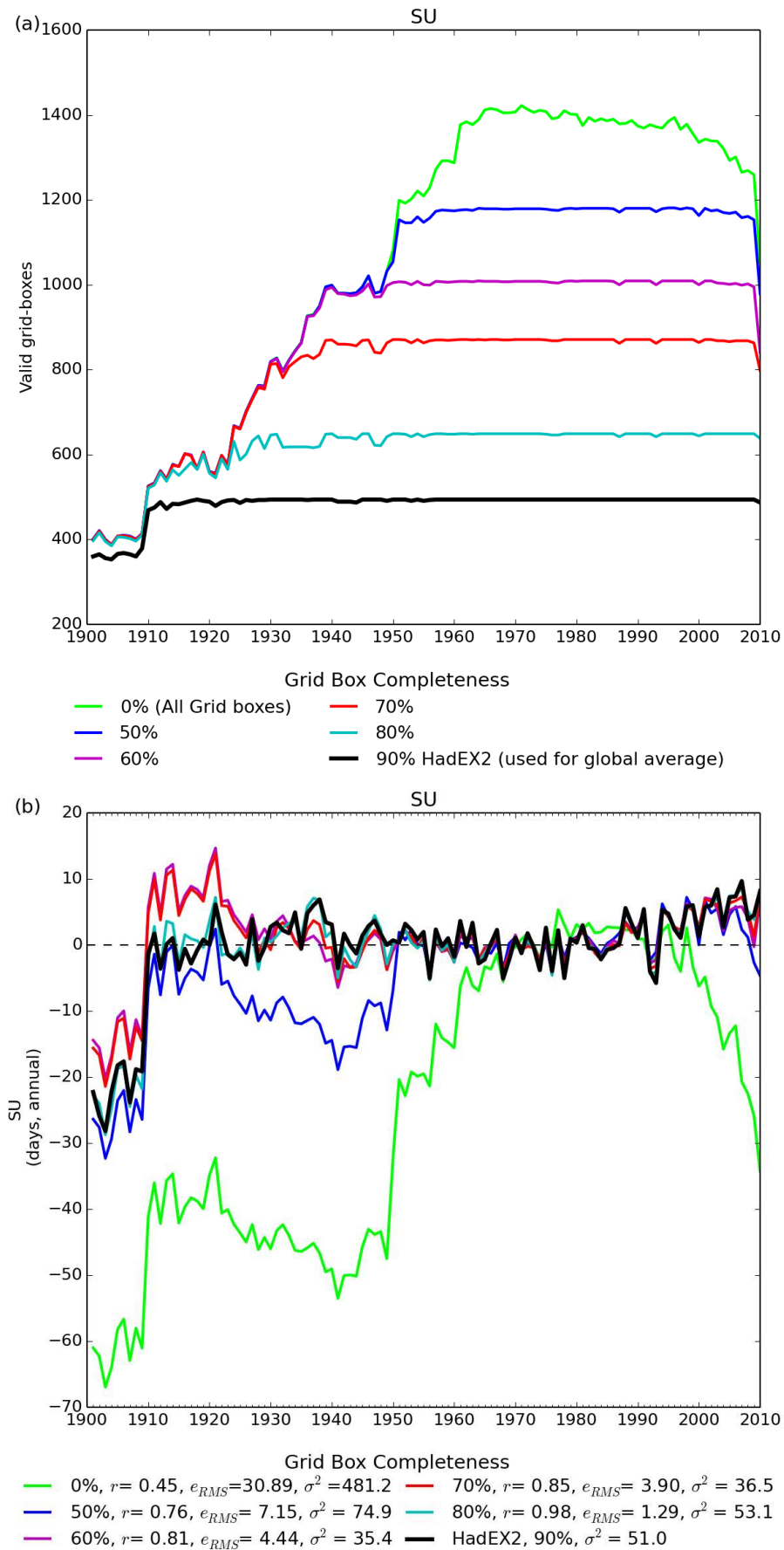
Figure 1: (a) The coverage, showing the different curves for different completeness requirements, for SU. The total coverage is shown the curve in light green, whereas the coverage used when calculating global averages is in black, with a range of other completeness percentages shown in between. (b) : The time series for global average of SU. Also shown are the comparison of other completenesses to that used in HadEX2 (90 %) using the correlation coefficient, r , the root mean square error e_{ems} and the variance, \sigma^2 .
