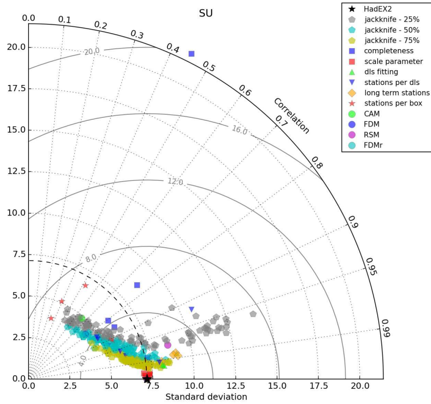
Figure 19: The Taylor Diagram for SU calculated using the global average timeseries for each choice. Each of the different methodological choices are shown using a different symbol and colour as indicated in the legend.
