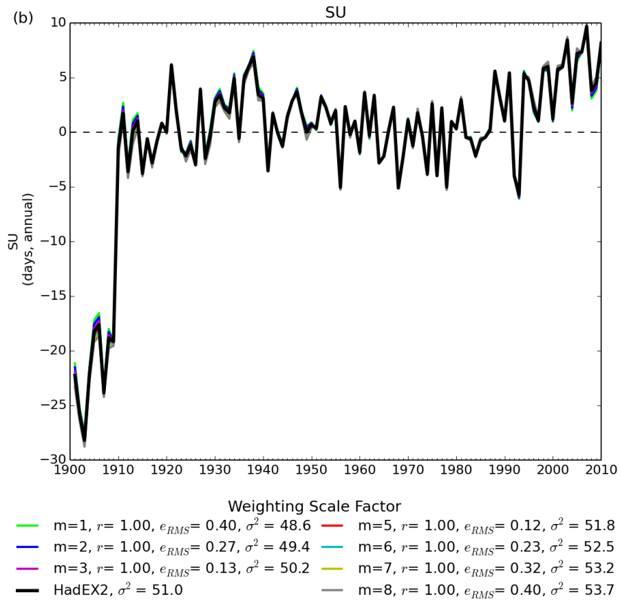
Figure 2: The time series for global average SU showing the different curves for the different weighting values (colours are indicated below the plot). The figure also shows the correlation coefficient ( r ), variance ( \sigma^2 ) and root-mean-square error ( e_{RMS} ) between each series and HadEX2. All choices have been normalised over the 1961-1990 period.
