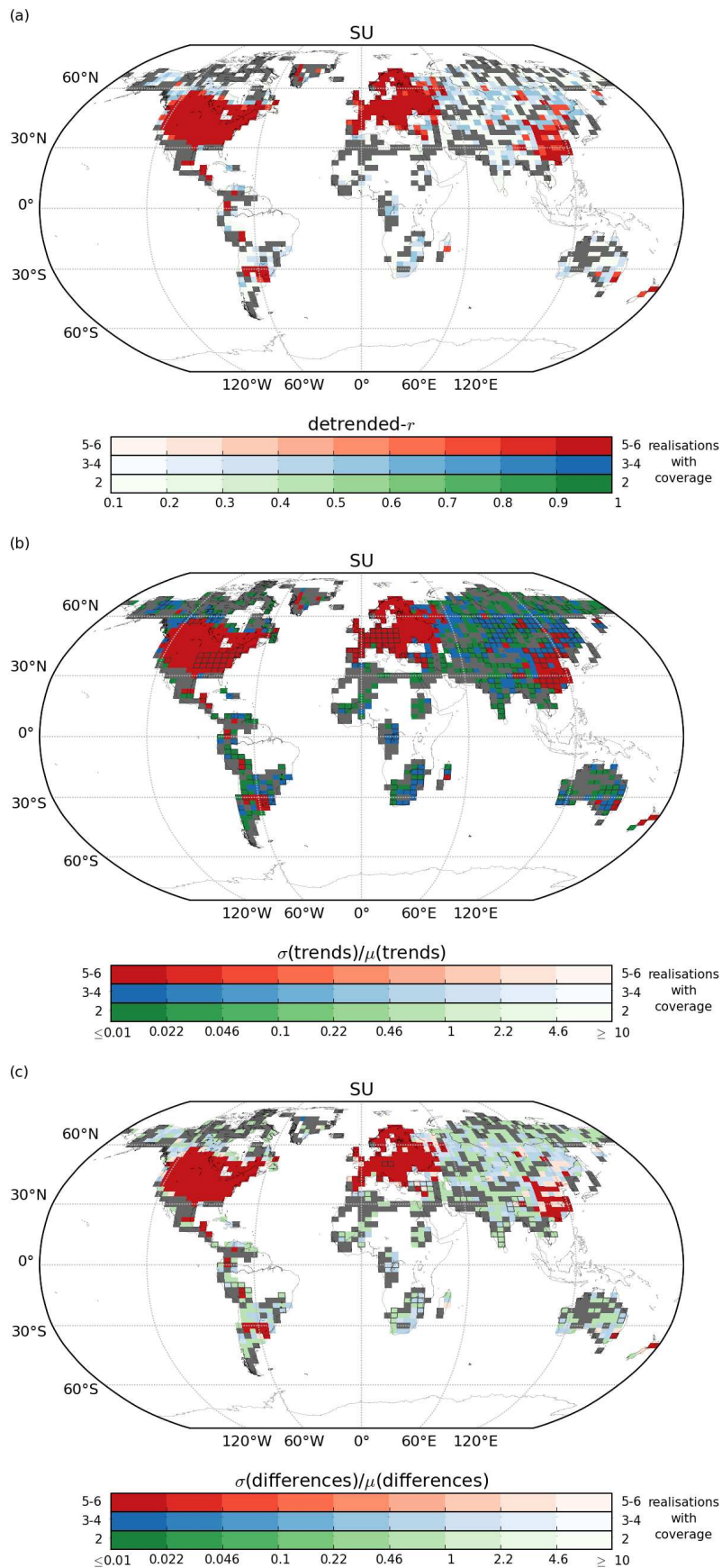
Figure 6: As for Fig. 4 but for SU restricted by the number of stations within a grid box. Grey grid boxes are those where only one of the 6 possible stations per grid box choices results in a value, green when 2, blue when 3-4 and red when 5-6 of the possible choices result in a value. Note that the HadEX2 method does not require any stations to be present within a grid box for a value to be calculated. In (b) and (c), boxes which have been outlined are ones where the trend was significant in the HadEX2 version. For details on the calculation method, see text.
