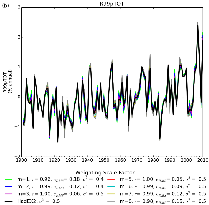
Figure 2: The time series for global average R99pTOT showing the different curves for the different weighting values (colours are indicated below the plot). The figure also shows the correlation coefficient ( r ), variance ( \sigma^2 ) and root-mean-square error ( e_{RMS} ) between each series and HadEX2. All choices have been normalised over the 1961-1990 period.
