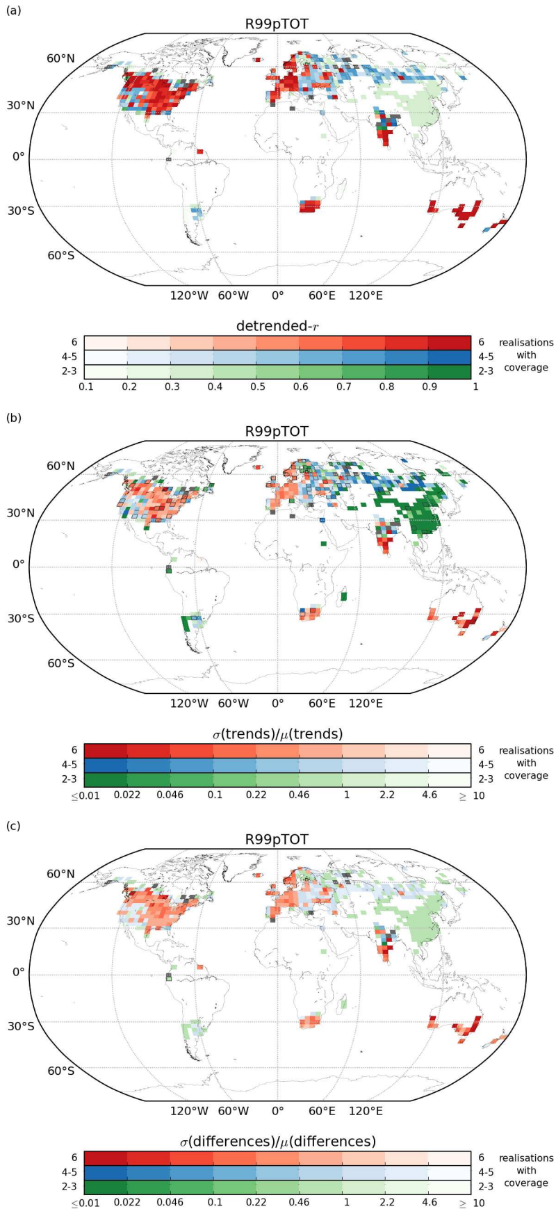
Figure 10: As for Fig. 4 but for long-term stations. Grey grid boxes are those where only one of the 6 possible station reporting length choices result in a value, green when 2-3, blue when 4-5 and red when 6 of the possible choices result in a value. In (b) and (c), boxes which have been outlined are ones where the trend was significant in the HadEX2 version. For details on the calculation method, see text.
