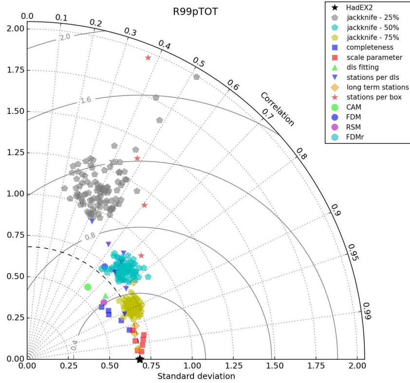
Figure 19: The Taylor Diagram for R99pTOT calculated using the global average timeseries for each choice. Each of the different methodological choices are shown using a different symbol and colour as indicated in the legend.
