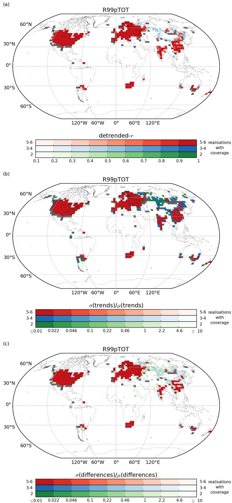
Figure 6: As for Fig. 4 but for R99pTOT restricted by the number of stations within a grid box. Grey grid boxes are those where only one of the 6 possible stations per grid box choices results in a value, green when 2, blue when 3-4 and red when 5-6 of the possible choices result in a value. Note that the HadEX2 method does not require any stations to be present within a grid box for a value to be calculated. In (b) and (c), boxes which have been outlined are ones where the trend was significant in the HadEX2 version. For details on the calculation method, see text.
