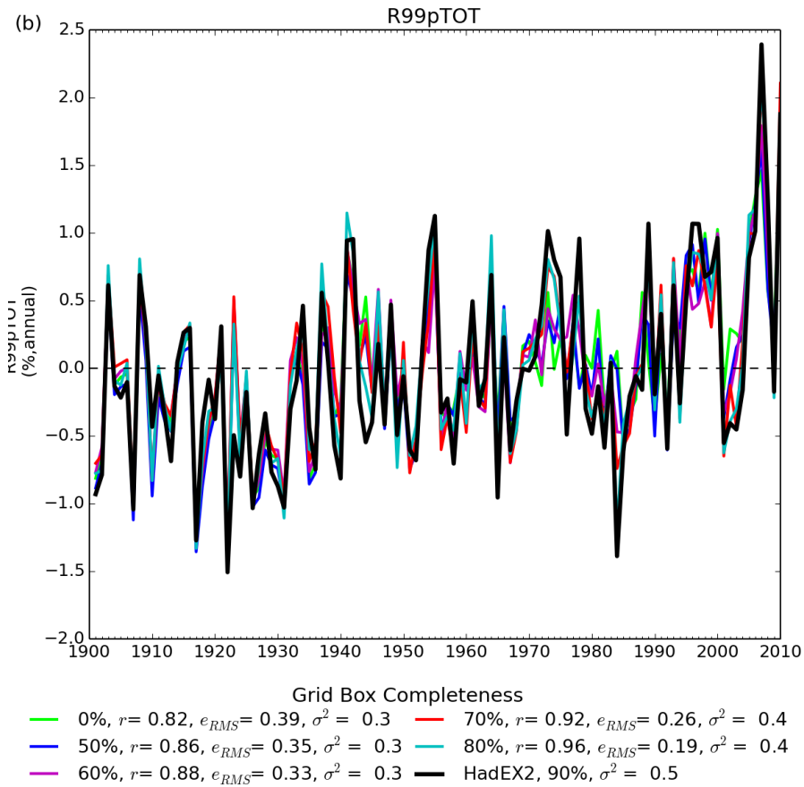
Figure 1: (a) The coverage, showing the different curves for different completeness requirements, for R99pTOT. The total coverage is shown the curve in light green, whereas the coverage used when calculating global averages is in black, with a range of other completeness percentages shown in between. (b) : The time series for global average of R99pTOT. Also shown are the comparison of other completenesses to that used in HadEX2 (90 %) using the correlation coefficient, r , the root mean square error e_{ems} and the variance, \sigma^2 .
