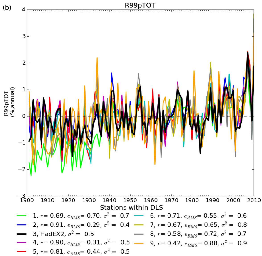
Figure 3: (a) : The number of non-missing grid boxes for R99pTOT showing the different curves for left numbers of stations within a DLS of the grid box centre. Note that the global average only takes grid boxes which have 90 per cent completeness or more, whereas all grid boxes are shown in the coverage series. (b) : The time series for global average R99pTOT.
