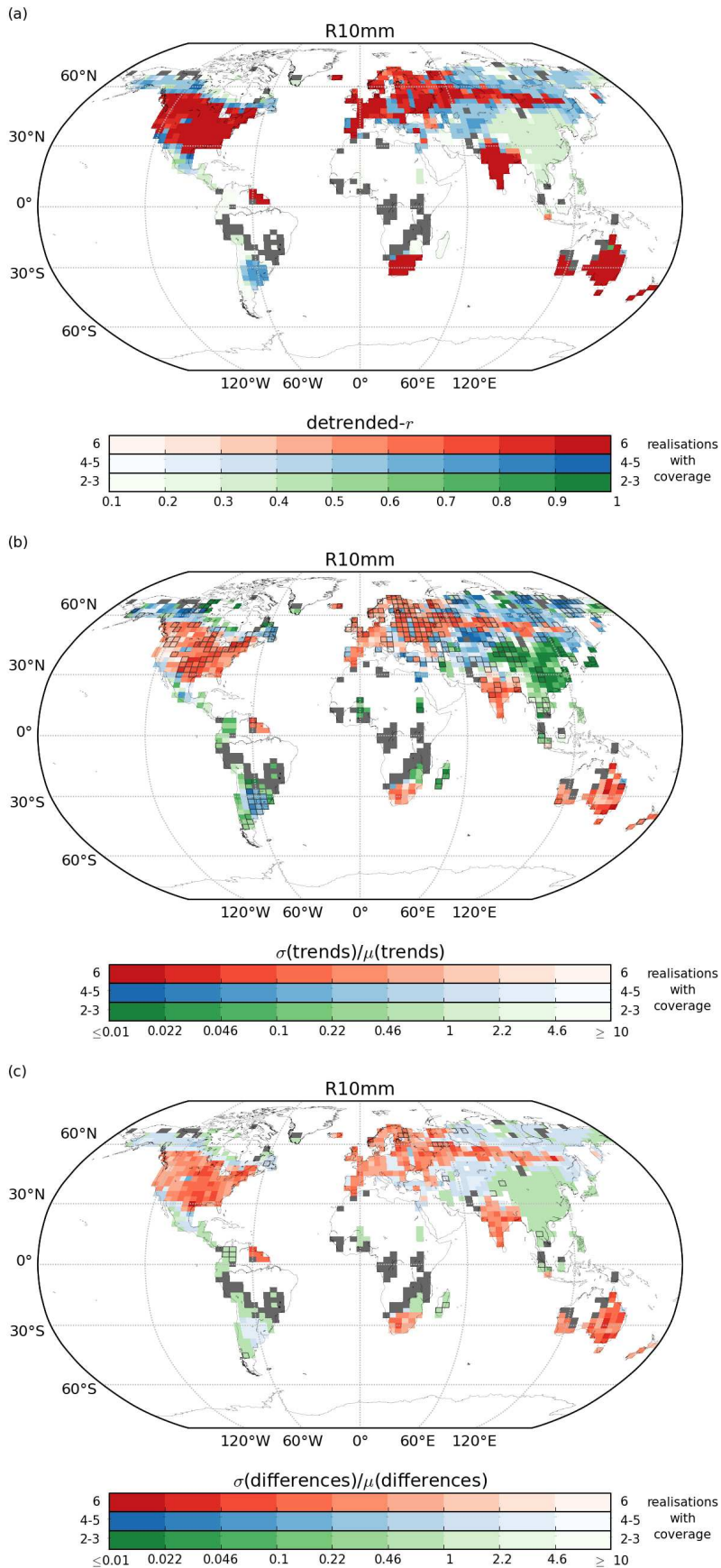
Figure 10: As for Fig. 4 but for long-term stations. Grey grid boxes are those where only one of the 6 possible station reporting length choices in a value, green when 2-3, blue when 4-5 and red when 6 of the possible choices result in a value. In (b) and (c), boxes which have been outlined are ones where the trend was significant in the HadEX2 version. For details on the calculation method, see text.
