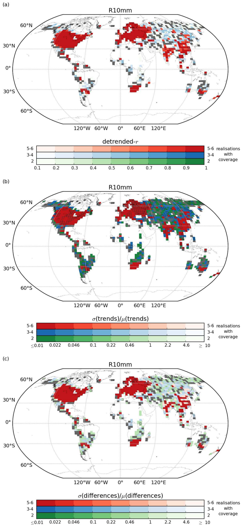
Figure 6: As for Fig. 4 but for R10mm restricted by the number of stations within a grid box. Grey grid boxes are those where only one of the 6 possible stations per grid box choices results in a value, green when 2, blue when 3-4 and red when 5-6 of the possible choices result in a value. Note that the HadEX2 method does not require any stations to be present within a grid box for a value to be calculated. In (b) and (c), boxes which have been outlined are ones where the trend was significant in the HadEX2 version. For details on the calculation method, see text.
