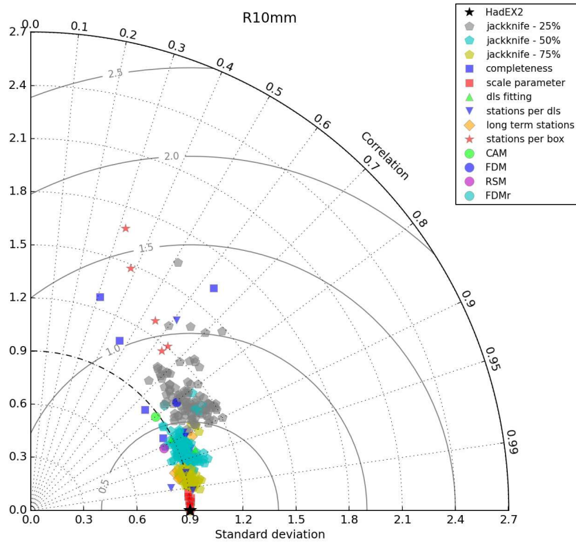
Figure 19: The Taylor Diagram for R10mm calculated using the global average timeseries for each choice. Each of the different methodological choices are shown using a different symbol and colour as indicated in the legend.
