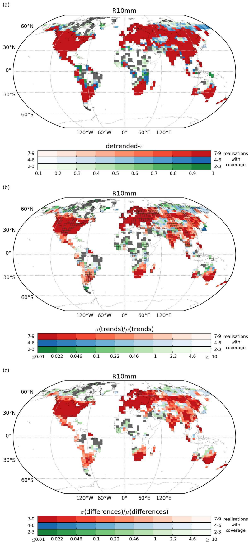
Figure 4: (a) : The mean detrended correlation coefficient, r for all the grid boxes; (b) : the standard deviation of the trends normalised by the mean trend ( \sigma/\mu ) calculated for the period 1951 to 2010, and (c) : the standard deviations of the differences normalised by the mean differences for R10mm, where the differences have been calculated between the averages over the periods 1991-2010 and 1951-1970. Grey grid boxes are those where only one of the 9 possible stations per DLS choices results in a value. The grid boxes are green when 2-3, blue when 4-6 and red when 7-9 of the possible choices result in a value. In (b) and (c), boxes which have been outlined are those where there is high confidence in a non-zero trend in HadEX2. For details on the calculation method, see text.
