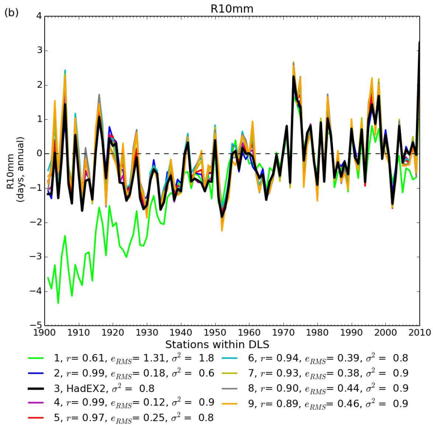
Figure 3: (a) : The number of non-missing grid boxes for R10mm showing the different curves for left numbers of stations within a DLS of the grid box centre. Note that the global average only takes grid boxes which have 90 per cent completeness or more, whereas all grid boxes are shown in the coverage series. (b) : The time series for global average R10mm.
