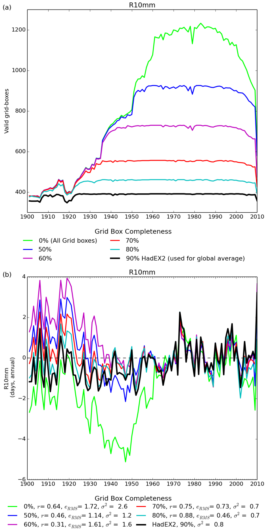
Figure 1: (a) The coverage, showing the different curves for different completeness requirements, for R10mm. The total coverage is shown the curve in light green, whereas the coverage used when calculating global averages is in black, with a range of other completeness percentages shown in between. (b) : The time series for global average of R10mm. Also shown are the comparison of other completenesses to that used in HadEX2 (90 %) using the correlation coefficient, r , the root mean square error e_{ems} and the variance, \sigma^2 .
