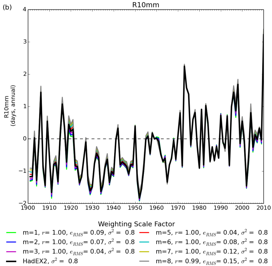
Figure 2: The time series for global average R10mm showing the different curves for the different weighting values (colours are indicated below the plot). The figure also shows the correlation coefficient ( r ), variance ( \sigma^2 ) and root-mean-square error ( e_{RMS} ) between each series and HadEX2. All choices have been normalised over the 1961-1990 period.
