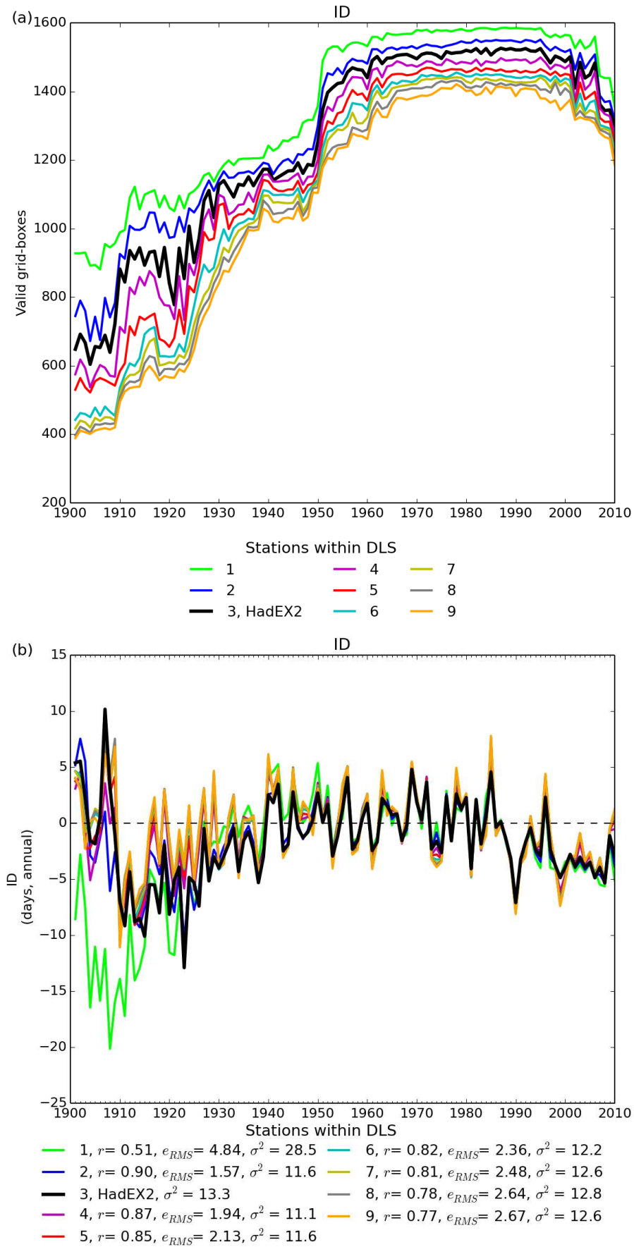
Figure 3: (a): The number of non-missing grid boxes for ID showing the different curves for left numbers of stations within a DLS of the grid box centre. Note that the global average only takes grid boxes which have 90 per cent completeness or more, whereas all grid boxes are shown in the coverage series. (b): The time series for global average ID.
