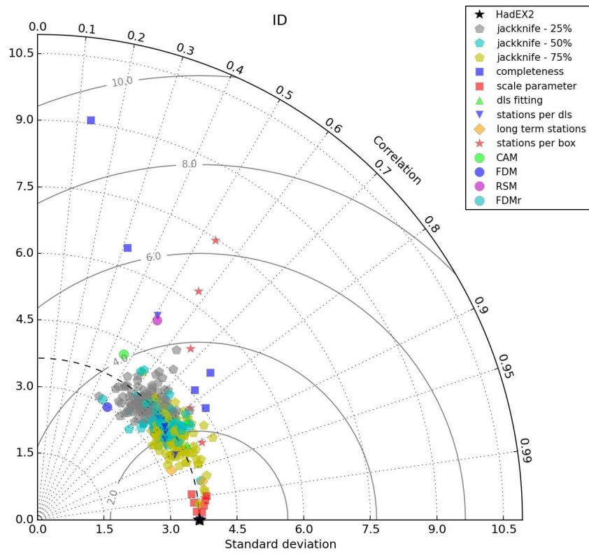
Figure 19: The Taylor Diagram for ID calculated using the global average timeseries for each choice. Each of the different methodological choices are shown using a different symbol and colour as indicated in the legend.
