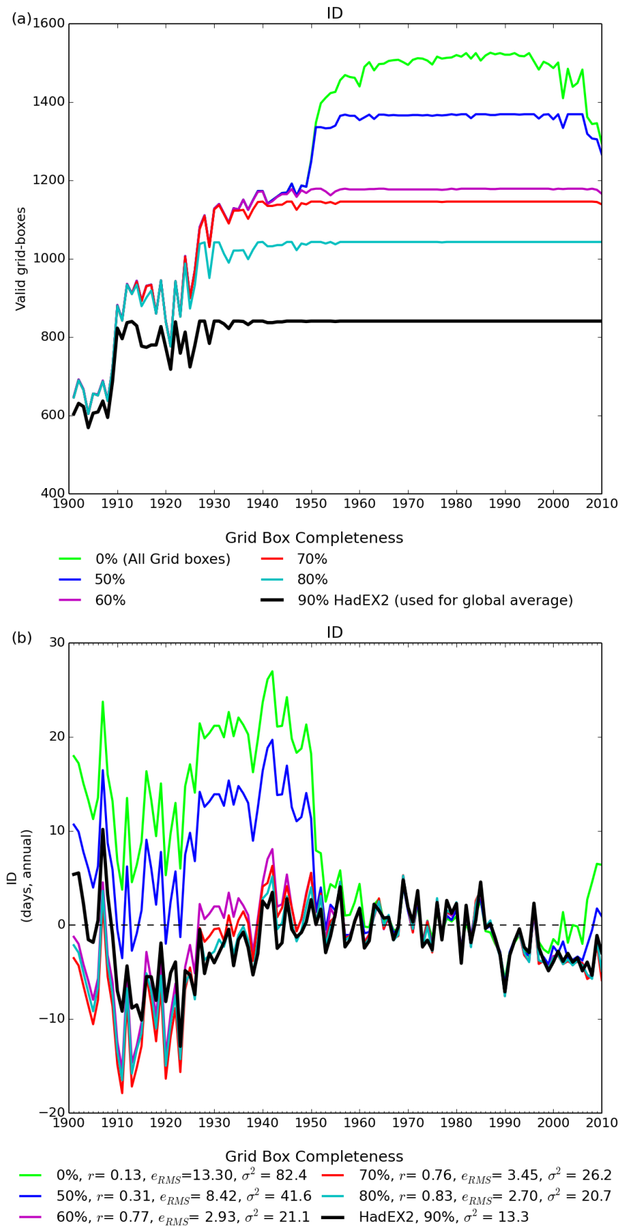
Figure 1: (a) The coverage, showing the different curves for different completeness requirements, for ID. The total coverage is shown the curve in light green, whereas the coverage used when calculating global averages is in black, with a range of other completeness percentages shown in between. (b) : The time series for global average of ID. Also shown are the comparison of other completenesses to that used in HadEX2 (90 %) using the correlation coefficient, r , the root mean square error e_{ems} and the variance, \sigma^2 .
