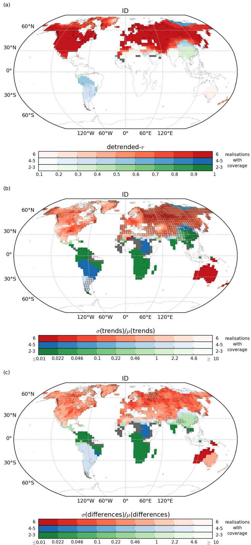
Figure 10: As for Fig. 4 but for long-term stations. Grey grid boxes are those where only one of the 6 possible station reporting length choices result in a value, green when 2-3, blue when 4-5 and red when 6 of the possible choices result in a value. In (b) and (c), boxes which have been outlined are ones where the trend was significant in the HadEX2 version. For details on the calculation method, see text.
