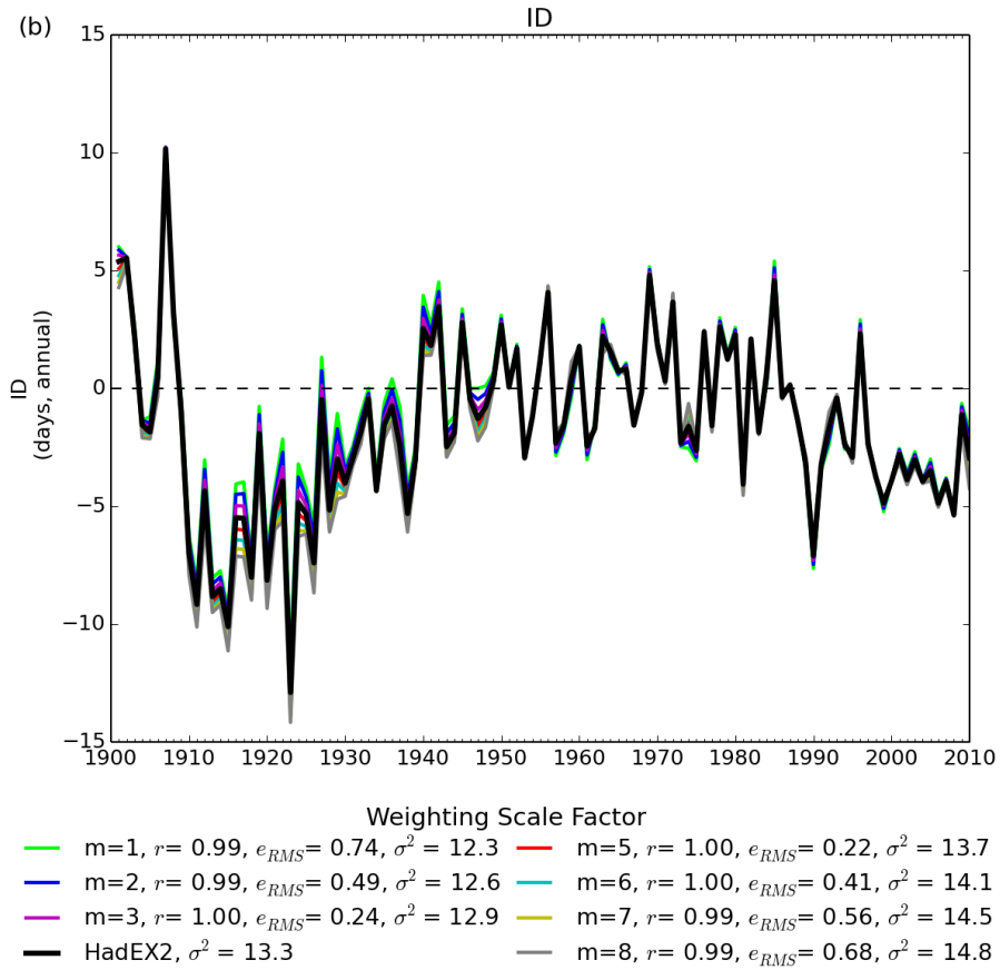
Figure 2: The time series for global average ID showing the different curves for the different weighting values (colours are indicated below the plot). The figure also shows the correlation coefficient ( r ), variance ( \sigma^2 ) and root-mean-square error ( e_{RMS} ) between each series and HadEX2. All choices have been normalised over the 1961-1990 period.
