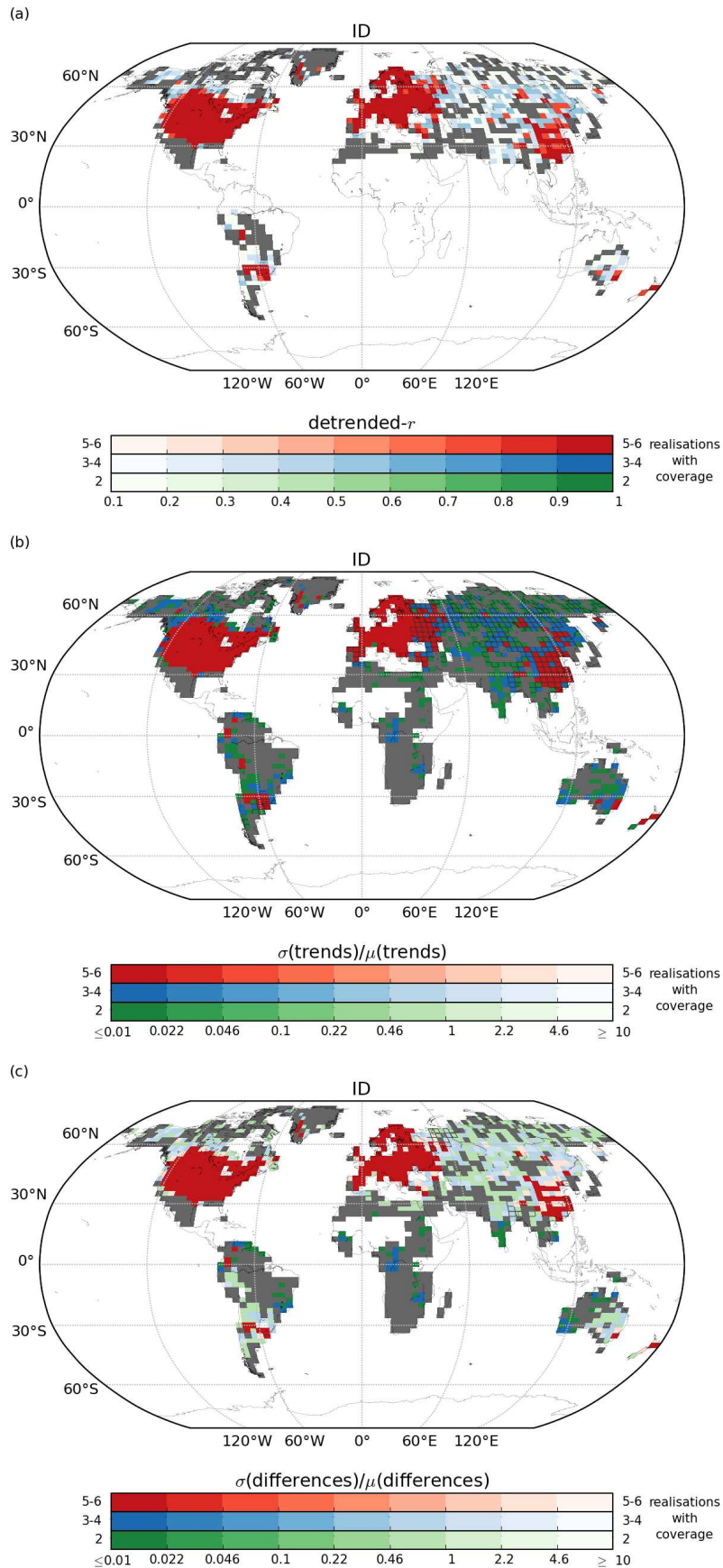
Figure 6: As for Fig. 4 but for ID restricted by the number of stations within a grid box. Grey grid boxes are those where only one of the 6 possible stations per grid box choices results in a value, green when 2, blue when 3-4 and red when 5-6 of the possible choices result in a value. Note that the HadEX2 method does not require any stations to be present within a grid box for a value to be calculated. In (b) and (c), boxes which have been outlined are ones where the trend was significant in the HadEX2 version. For details on the calculation method, see text.
