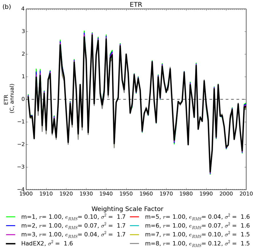
Figure 2: The time series for global average ETR showing the different curves for the different weighting values (colours are indicated below the plot). The figure also shows the correlation coefficient ( r ), variance ( \sigma^2 ) and root-mean-square error ( e_{RMS} ) between each series and HadEX2. All choices have been normalised over the 1961-1990 period.
