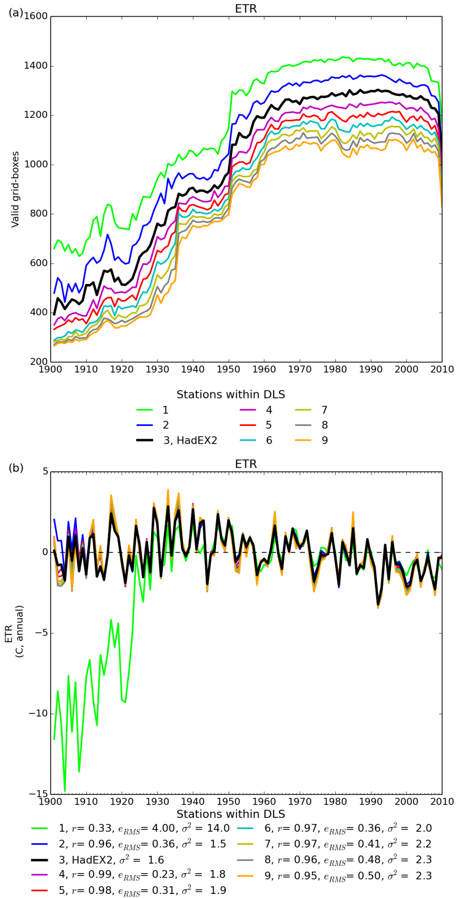
Figure 3: (a) : The number of non-missing grid boxes for ETR showing the different curves for left numbers of stations within a DLS of the grid box centre. Note that the global average only takes grid boxes which have 90 per cent completeness or more, whereas all grid boxes are shown in the coverage series. (b) : The time series for global average ETR.
