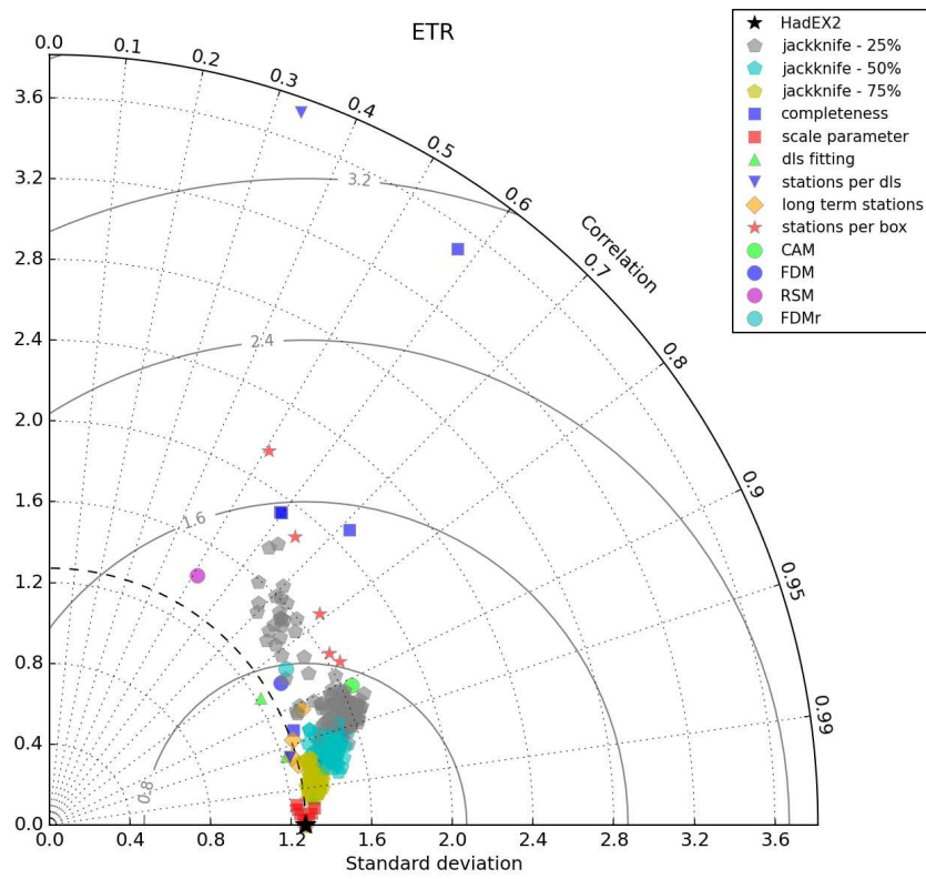
Figure 19: The Taylor Diagram for ETR calculated using the global average timeseries for each choice. Each of the different methodological choices are shown using a different symbol and colour as indicated in the legend.
