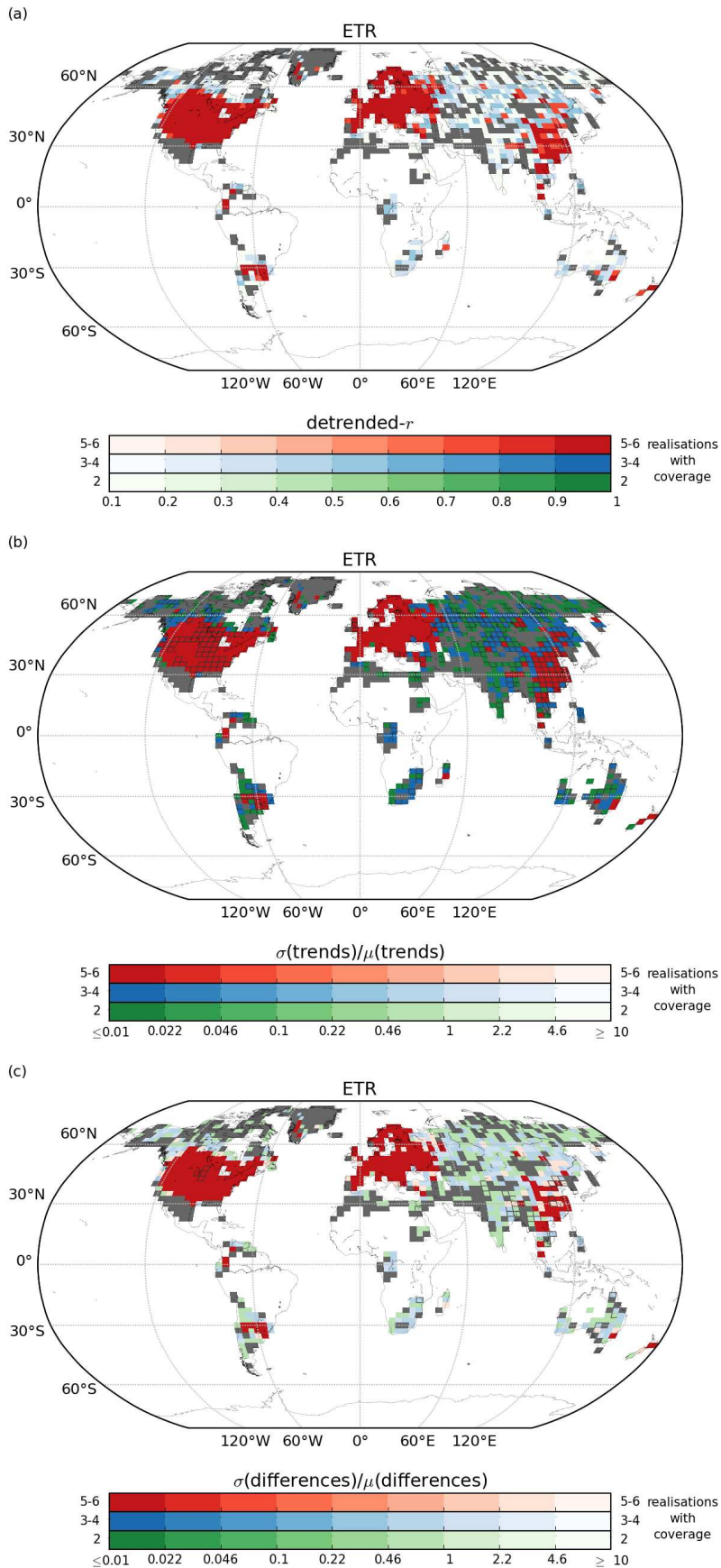
Figure 6: As for Fig. 4 but for ETR restricted by the number of stations within a grid box. Grey grid boxes are those where only one of the 6 possible stations per grid box choices results in a value, green when 2, blue when 3-4 and red when 5-6 of the possible choices result in a value. Note that the HadEX2 method does not require any stations to be present within a grid box for a value to be calculated. In (b) and (c), boxes which have been outlined are ones where the trend was significant in the HadEX2 version. For details on the calculation method, see text.
