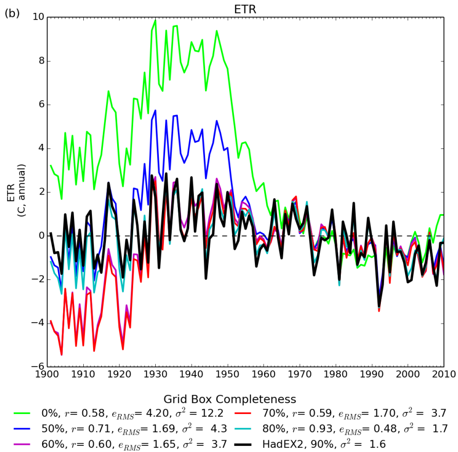
Figure 1: (a) The coverage, showing the different curves for different completeness requirements, for ETR. The total coverage is shown the curve in light green, whereas the coverage used when calculating global averages is in black, with a range of other completeness percentages shown in between. (b) : The time series for global average of ETR. Also shown are the comparison of other completenesses to that used in HadEX2 (90 %) using the correlation coefficient, r , the root mean square error e_{ems} and the variance, \sigma^2 .
