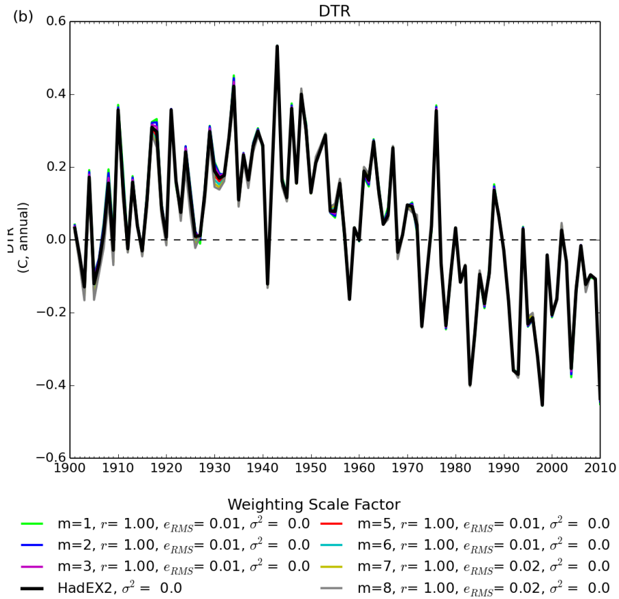
Figure 2: The time series for global average DTR showing the different curves for the different weighting values (colours are indicated below the plot). The figure also shows the correlation coefficient ( r ), variance ( \sigma^2 ) and root-mean-square error ( e_{RMS} ) between each series and HadEX2. All choices have been normalised over the 1961-1990 period.
