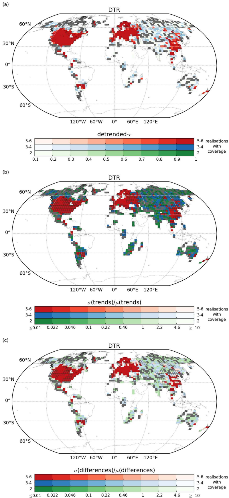
Figure 6: As for Fig. 4 but for DTR restricted by the number of stations within a grid box. Grey grid boxes are those where only one of the 6 possible stations per grid box choices results in a value, green when 2, blue when 3-4 and red when 5-6 of the possible choices result in a value. Note that the HadEX2 method does not require any stations to be present within a grid box for a value to be calculated. In (b) and (c), boxes which have been outlined are ones where the trend was significant in the HadEX2 version. For details on the calculation method, see text.
