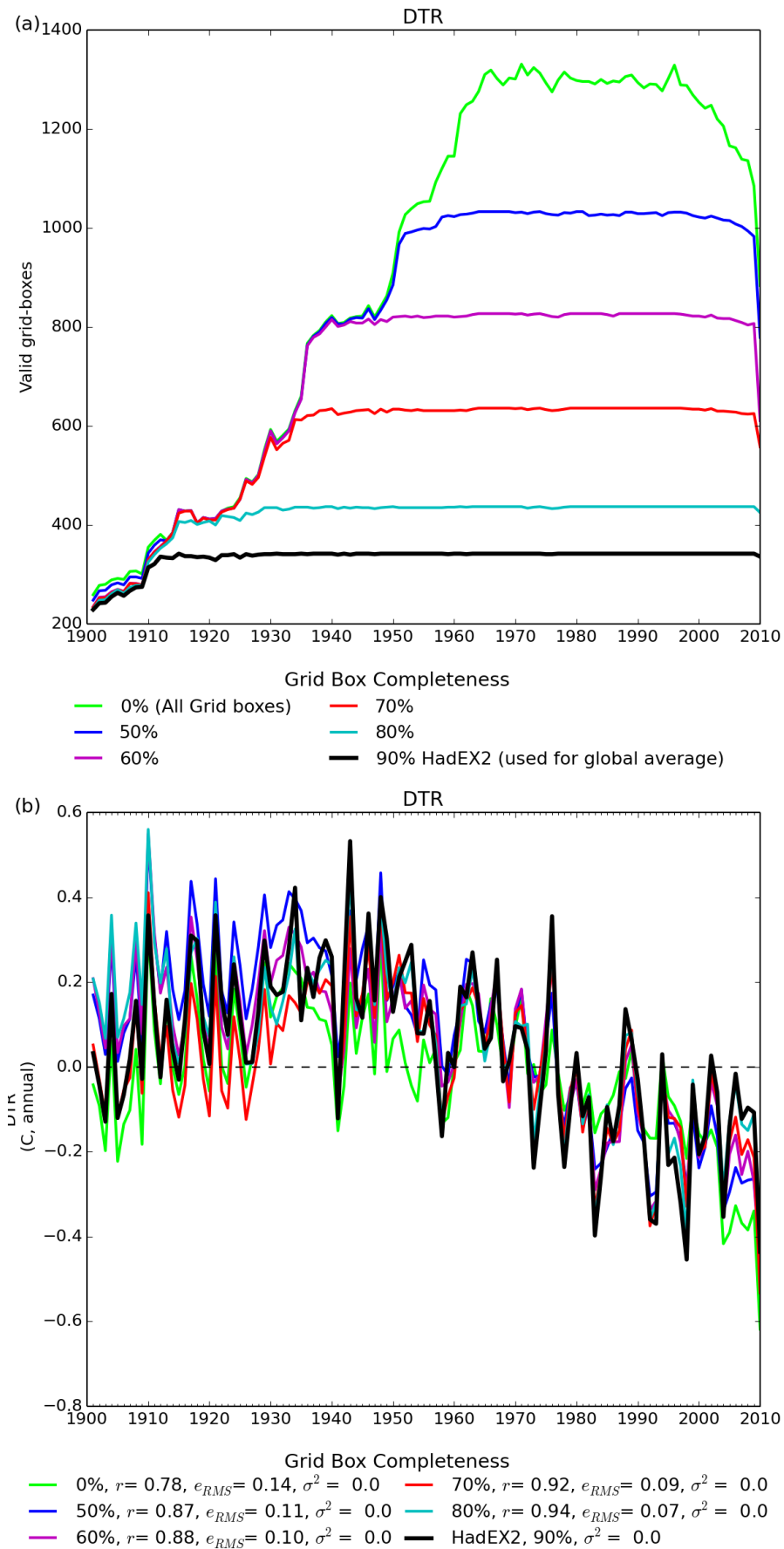
Figure 1: (a) The coverage, showing the different curves for different completeness requirements, for DTR. The total coverage is shown the curve in light green, whereas the coverage used when calculating global averages is in black, with a range of other completeness percentages shown in between. (b) : The time series for global average of DTR. Also shown are the comparison of other completenesses to that used in HadEX2 (90 %) using the correlation coefficient, r , the root mean square error e_{ems} and the variance, \sigma^2 .
