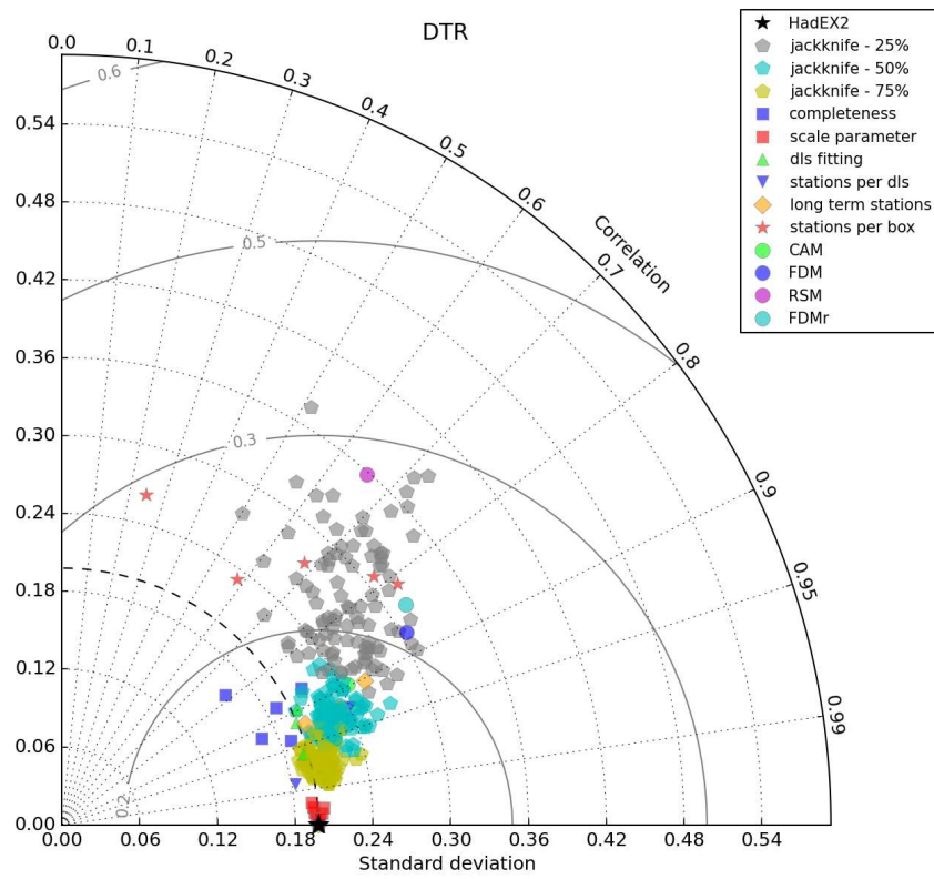
Figure 19: The Taylor Diagram for DTR calculated using the global average timeseries for each choice. Each of the different methodological choices are shown using a different symbol and colour as indicated in the legend.
