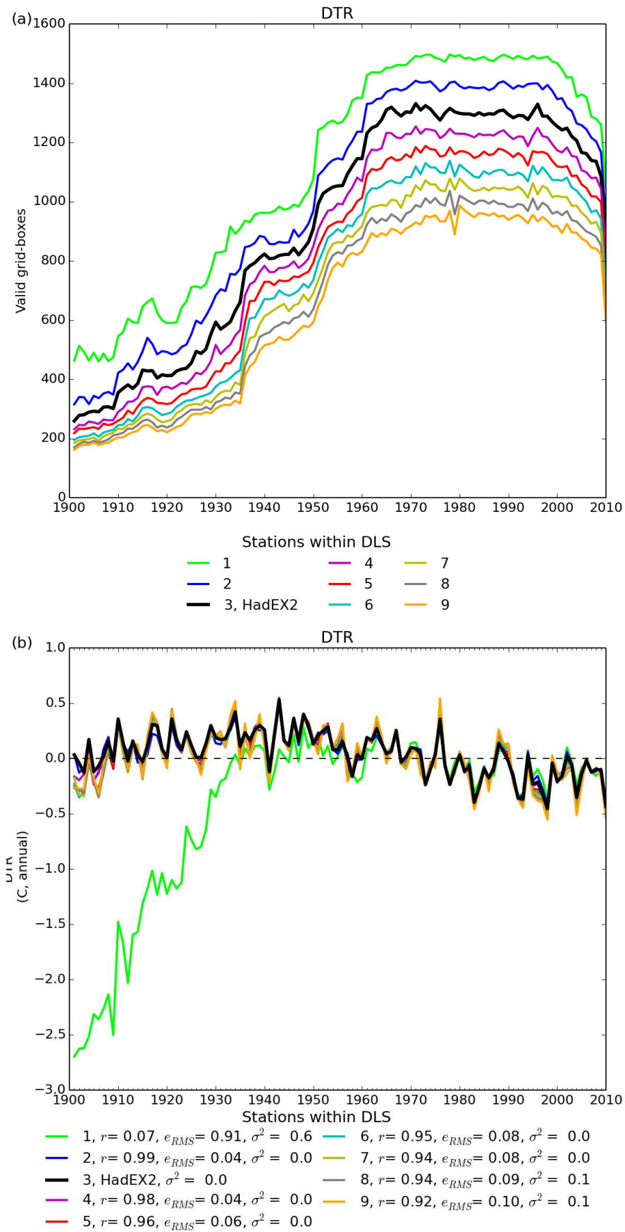
Figure 3: (a) : The number of non-missing grid boxes for DTR showing the different curves for left numbers of stations within a DLS of the grid box centre. Note that the global average only takes grid boxes which have 90 per cent completeness or more, whereas all grid boxes are shown in the coverage series. (b) : The time series for global average DTR.
