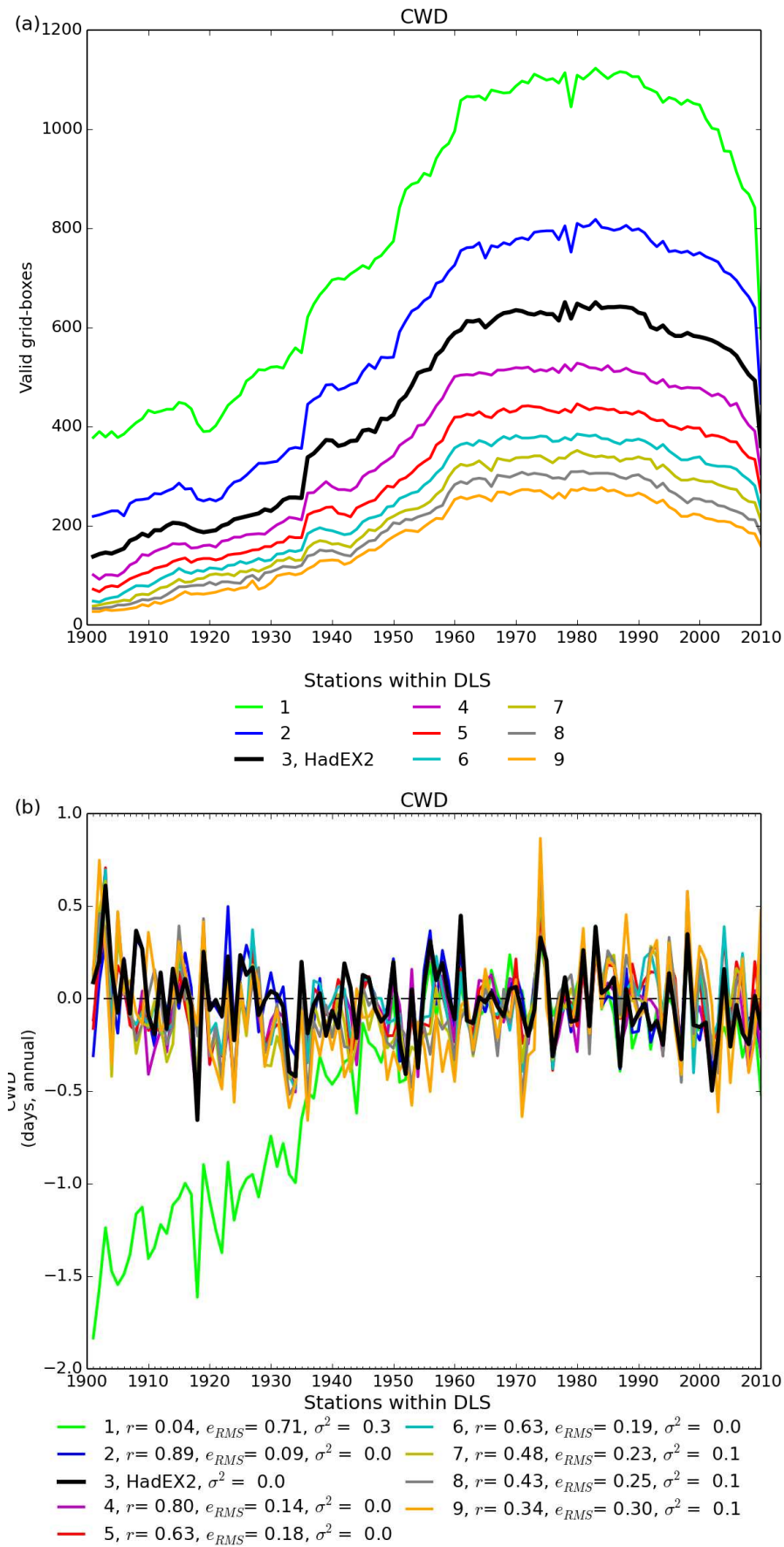
Figure 3: (a) : The number of non-missing grid boxes for CWD showing the different curves for left numbers of stations within a DLS of the grid box centre. Note that the global average only takes grid boxes which have 90 per cent completeness or more, whereas all grid boxes are shown in the coverage series. (b) : The time series for global average CWD.
