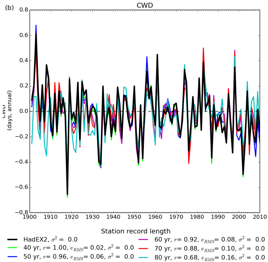
Figure 9: As for Fig. 3 but for long-term stations.
