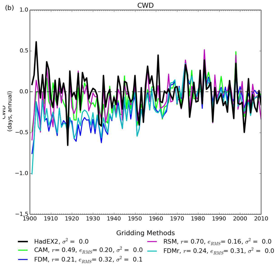
15 Figure 14: As for Fig. 3 but for the four different gridding methods.
