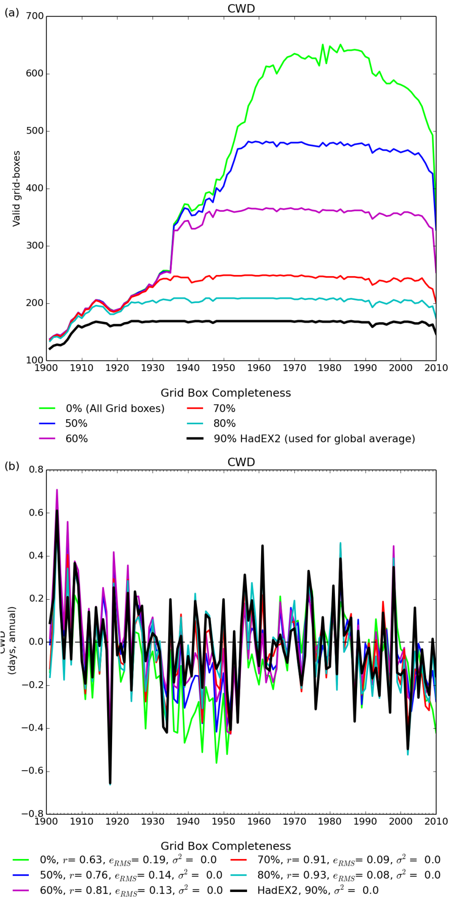
Figure 1: (a) The coverage, showing the different curves for different completeness requirements, for CWD. The total coverage is shown the curve in light green, whereas the coverage used when calculating global averages is in black, with a range of other completeness percentages shown in between. (b) : The time series for global average of CWD. Also shown are the comparison of other completenesses to that used in HadEX2 (90 %) using the correlation coefficient, r , the root mean square error e_{ems} and the variance, \sigma^2 .
