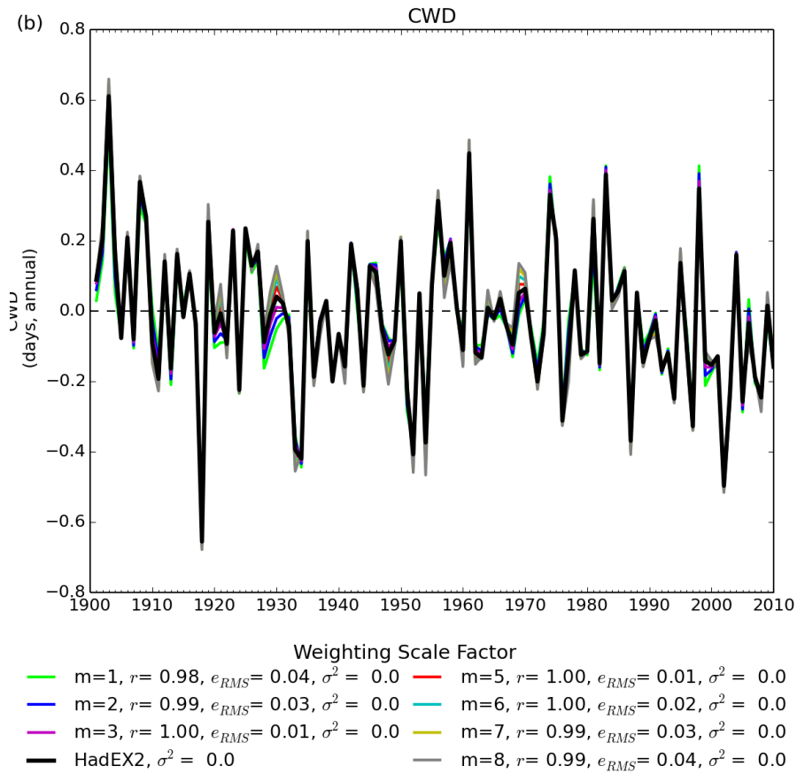
Figure 2: The time series for global average CWD showing the different curves for the different weighting values (colours are indicated below the plot). The figure also shows the correlation coefficient ( r ), variance ( \sigma^2 ) and root-mean-square error ( e_{RMS} ) between each series and HadEX2. All choices have been normalised over the 1961-1990 period.
