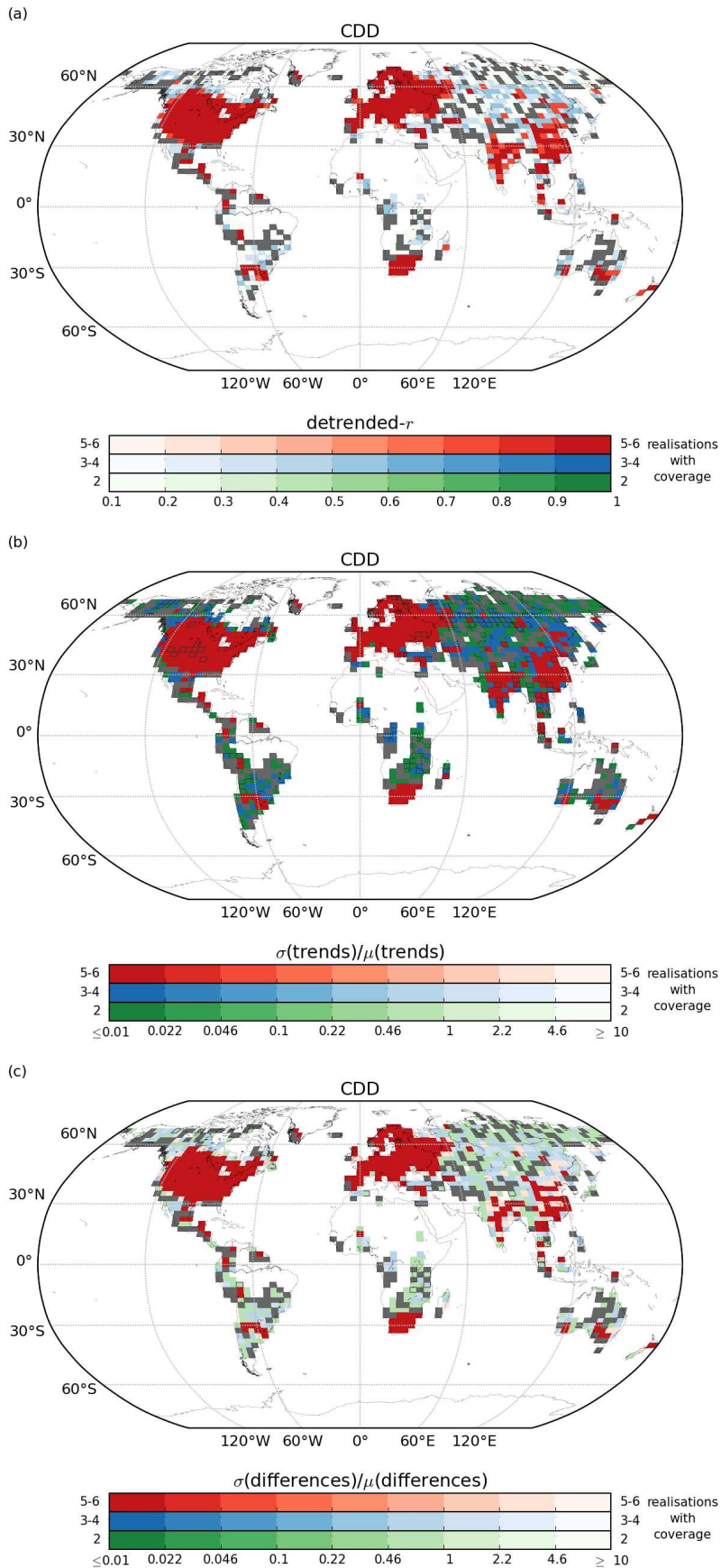
Figure 6: As for Fig. 4 but for CDD restricted by the number of stations within a grid box. Grey grid boxes are those where only one of the 6 possible stations per grid box choices results in a value, green when 2, blue when 3-4 and red when 5-6 of the possible choices result in a value. Note that the HadEX2 method does not require any stations to be present within a grid box for a value to be calculated. In (b) and (c), boxes which have been outlined are ones where the trend was significant in the HadEX2 version. For details on the calculation method, see text.
