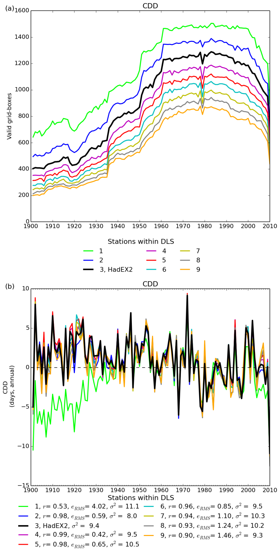
Figure 3: (a) : The number of non-missing grid boxes for CDD showing the different curves for left numbers of stations within a DLS of the grid box centre. Note that the global average only takes grid boxes which have 90 per cent completeness or more, whereas all grid boxes are shown in the coverage series. (b) : The time series for global average CDD.
