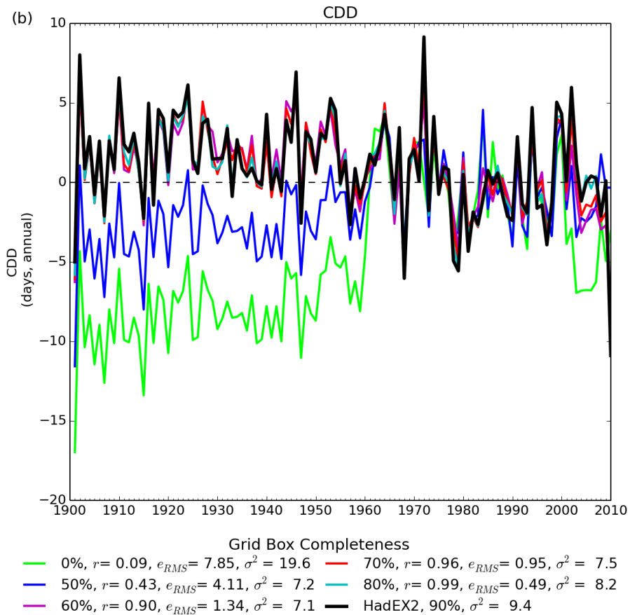
Figure 1: (a) The coverage, showing the different curves for different completeness requirements, for CDD. The total coverage is shown the curve in light green, whereas the coverage used when calculating global averages is in black, with a range of other completeness percentages shown in between. (b) : The time series for global average of CDD. Also shown are the comparison of other completenesses to that used in HadEX2 (90 %) using the correlation coefficient, r , the root mean square error e_{ems} and the variance, \sigma^2 .
