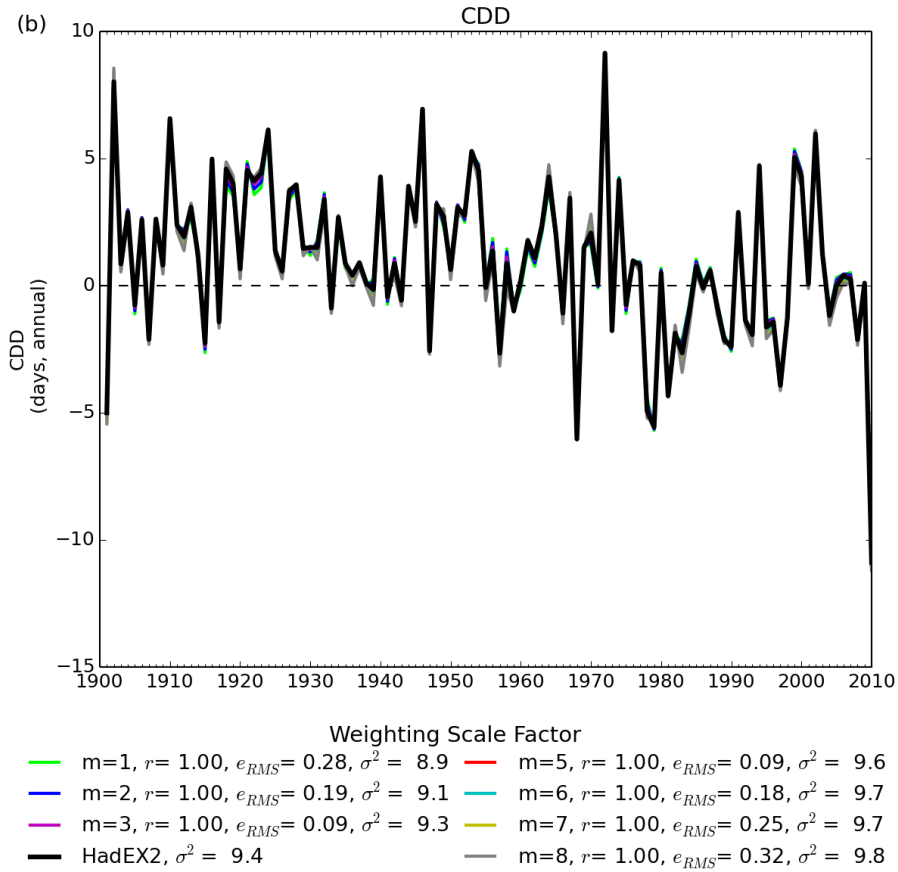
Figure 2: The time series for global average CDD showing the different curves for the different weighting values (colours are indicated below the plot). The figure also shows the correlation coefficient ( r ), variance ( \sigma^2 ) and root-mean-square error ( e_{RMS} ) between each series and HadEX2. All choices have been normalised over the 1961-1990 period.
