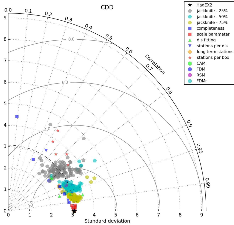
Figure 19: The Taylor Diagram for CDD calculated using the global average timeseries for each choice. Each of the different methodological choices are shown using a different symbol and colour as indicated in the legend.
